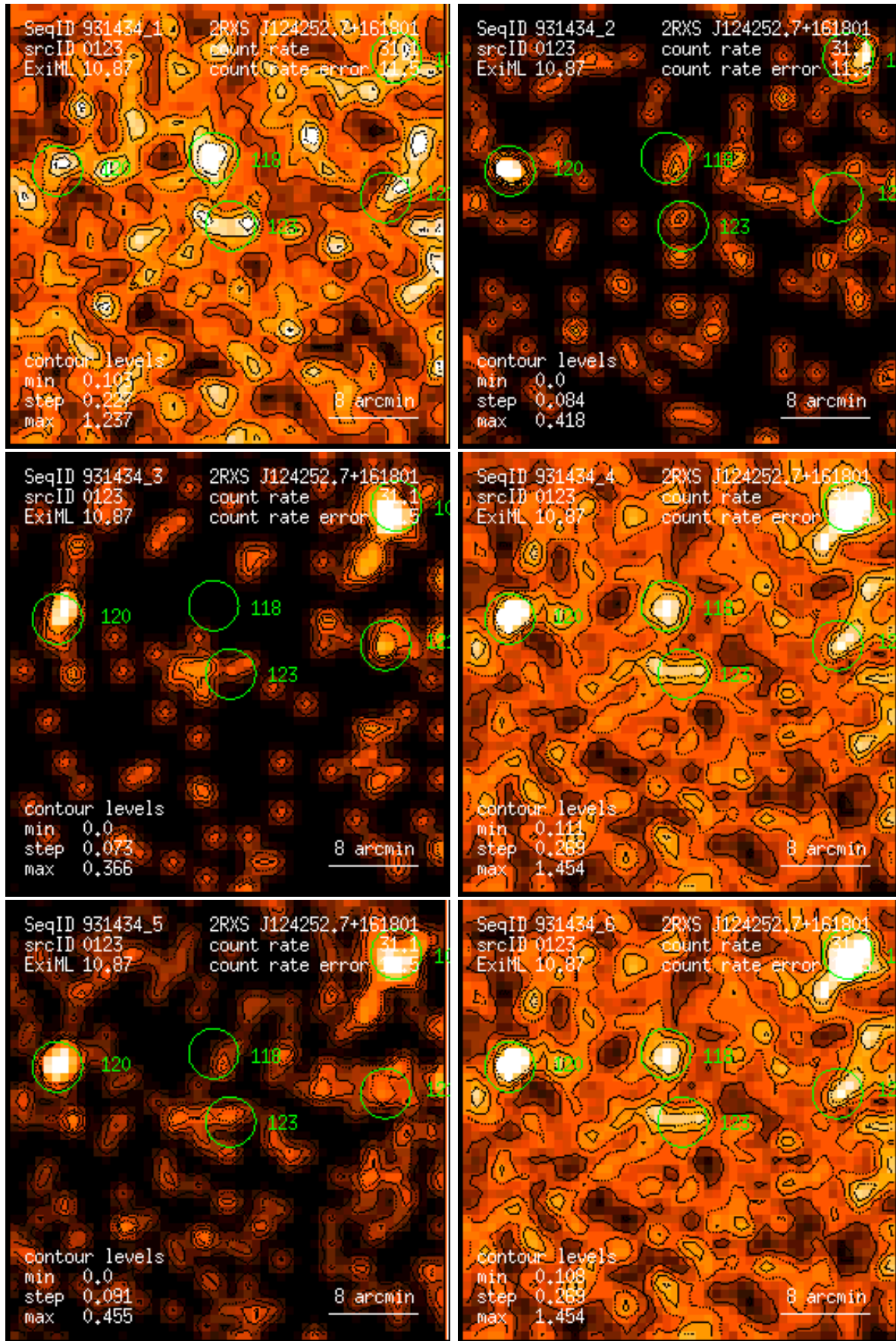
Figure 123: RASS 931434: detection 0123: band rate images, Gaussian filter: (1) PSPC channels 11 – 41, (2) 52 – 90, (3) 91 – 201, (4) 11 – 235, (5) 52 – 201, (6) 11 – 201. Broad band rates in counts/ks. Band rate contour levels in counts/ks/arcmin 2 .
