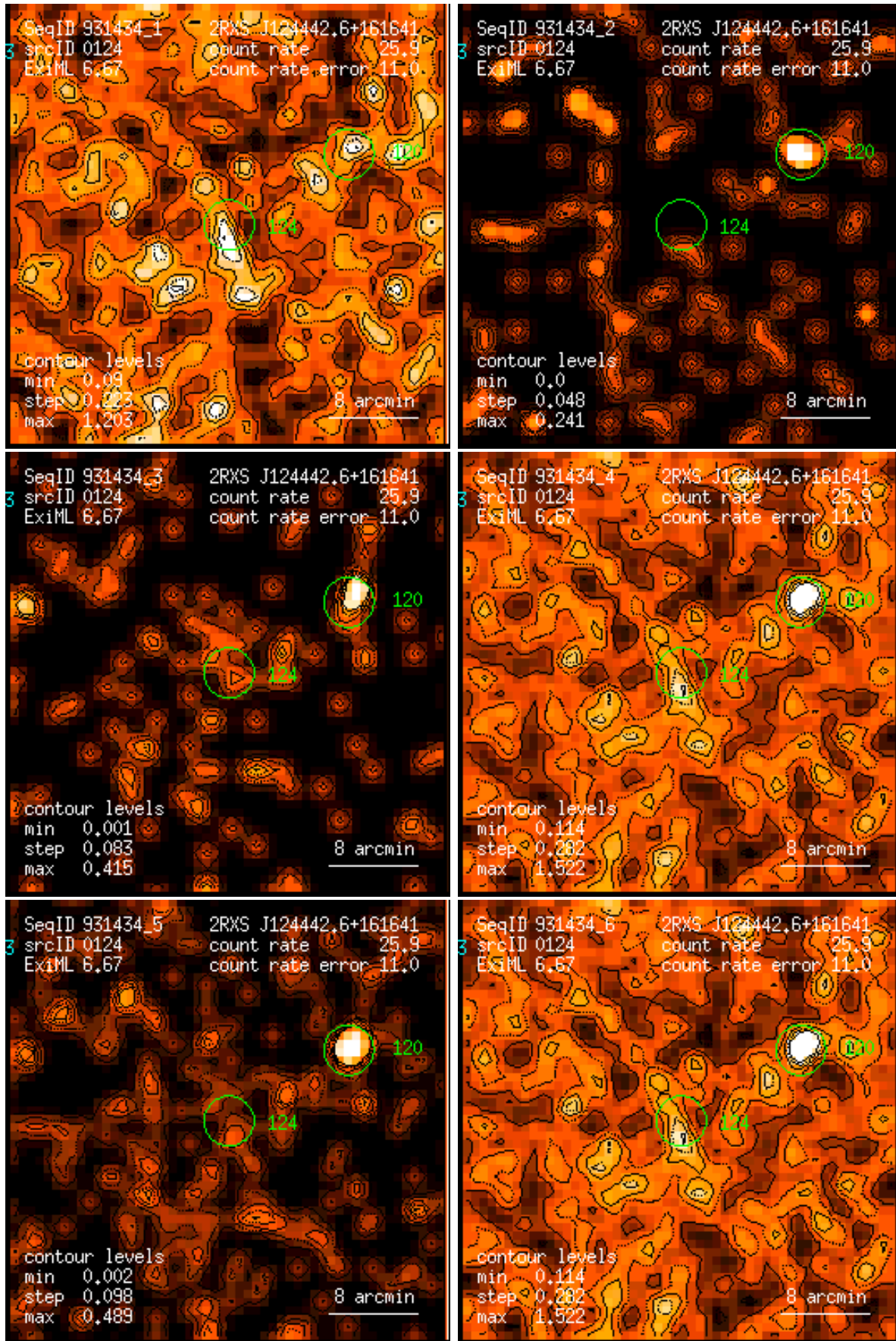
Figure 124: RASS 931434: detection 0124: band rate images, Gaussian filter: (1) PSPC channels 11 – 41, (2) 52 – 90, (3) 91 – 201, (4) 11 – 235, (5) 52 – 201, (6) 11 – 201. Broad band rates in counts/ks. Band rate contour levels in counts/ks/arcmin 2 .
