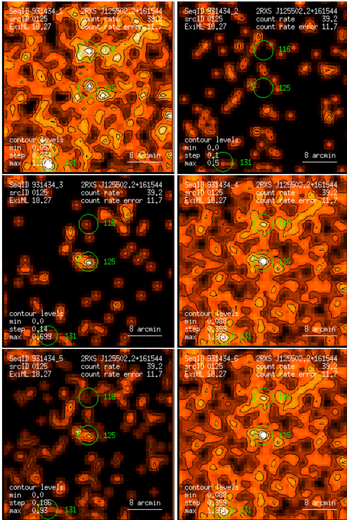
Figure 125: RASS 931434: detection 0125: band rate images, Gaussian filter: (1) PSPC channels 11 – 41, (2) 52 – 90, (3) 91 – 201, (4) 11 – 235, (5) 52 – 201, (6) 11 – 201. Broad band rates in counts/ks. Band rate contour levels in counts/ks/arcmin 2 .
