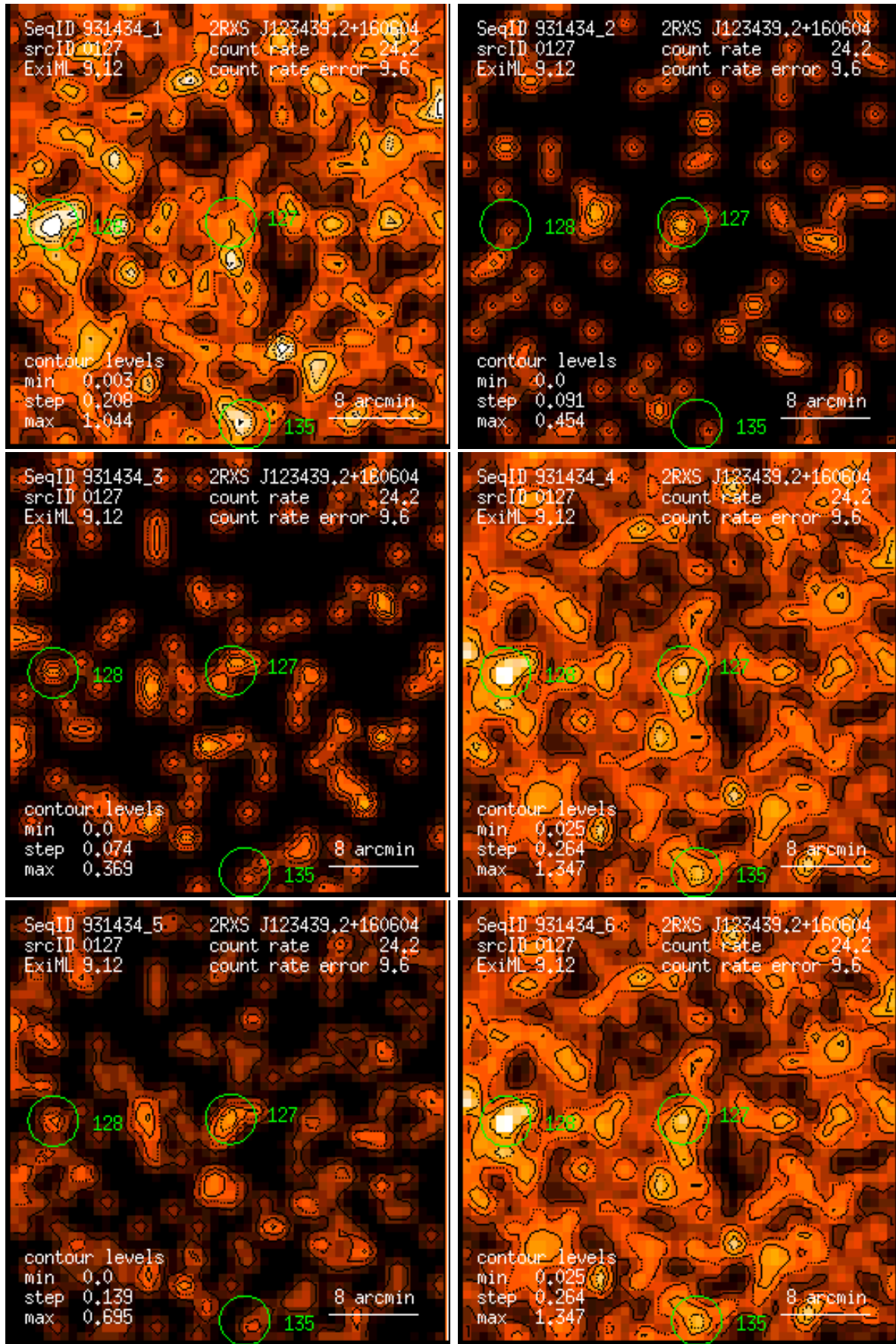
Figure 127: RASS 931434: detection 0127: band rate images, Gaussian filter: (1) PSPC channels 11 – 41, (2) 52 – 90, (3) 91 – 201, (4) 11 – 235, (5) 52 – 201, (6) 11 – 201. Broad band rates in counts/ks. Band rate contour levels in counts/ks/arcmin 2 .
