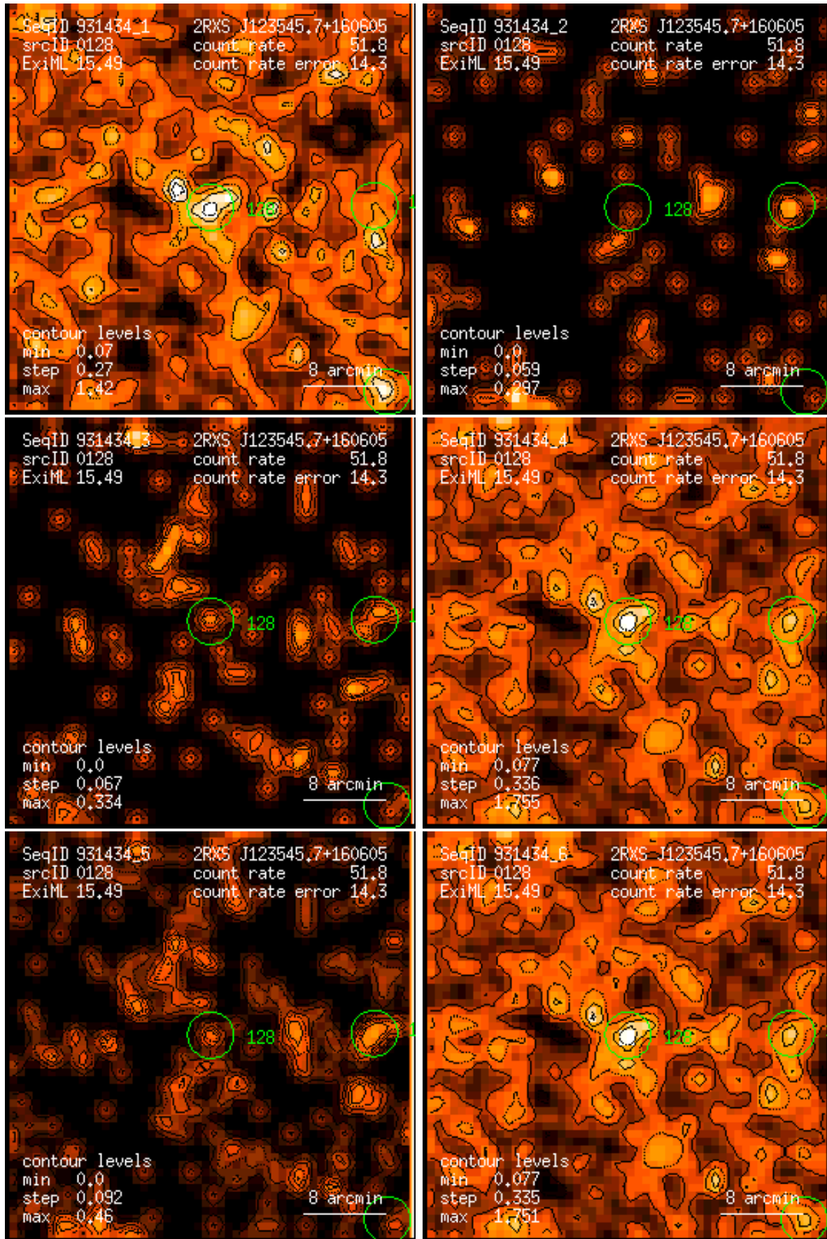
Figure 128: RASS 931434: detection 0128: band rate images, Gaussian filter: (1) PSPC channels 11 – 41, (2) 52 – 90, (3) 91 – 201, (4) 11 – 235, (5) 52 – 201, (6) 11 – 201. Broad band rates in counts/ks. Band rate contour levels in counts/ks/arcmin 2 .
