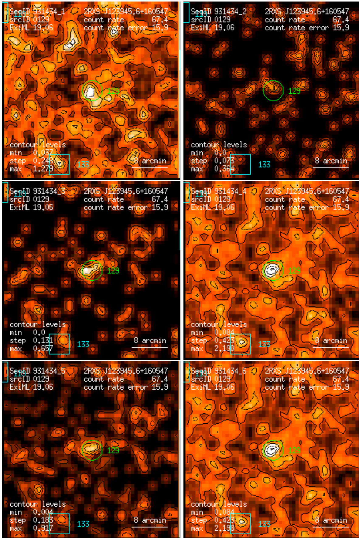
Figure 129: RASS 931434: detection 0129: band rate images, Gaussian filter: (1) PSPC channels 11 – 41, (2) 52 – 90, (3) 91 – 201, (4) 11 – 235, (5) 52 – 201, (6) 11 – 201. Broad band rates in counts/ks. Band rate contour levels in counts/ks/arcmin 2 .
