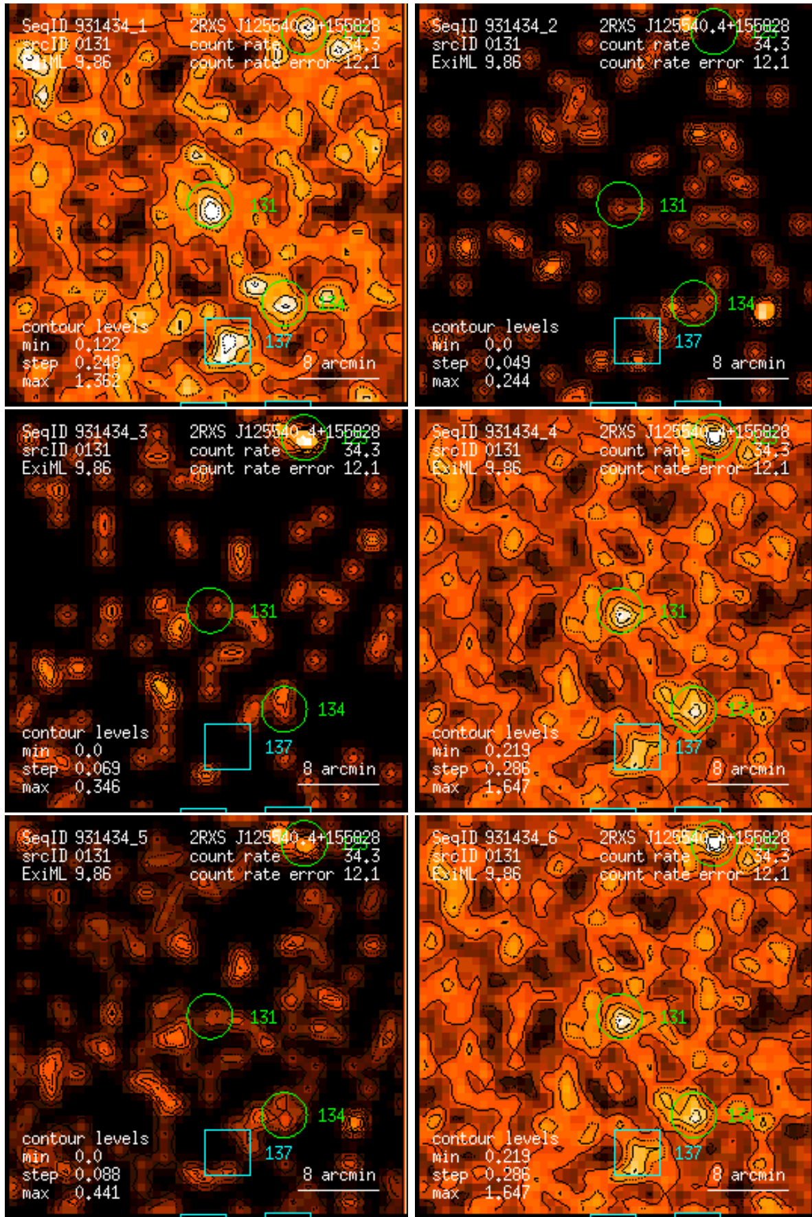
Figure 131: RASS 931434: detection 0131: band rate images, Gaussian filter: (1) PSPC channels 11 – 41, (2) 52 – 90, (3) 91 – 201, (4) 11 – 235, (5) 52 – 201, (6) 11 – 201. Broad band rates in counts/ks. Band rate contour levels in counts/ks/arcmin 2 .
