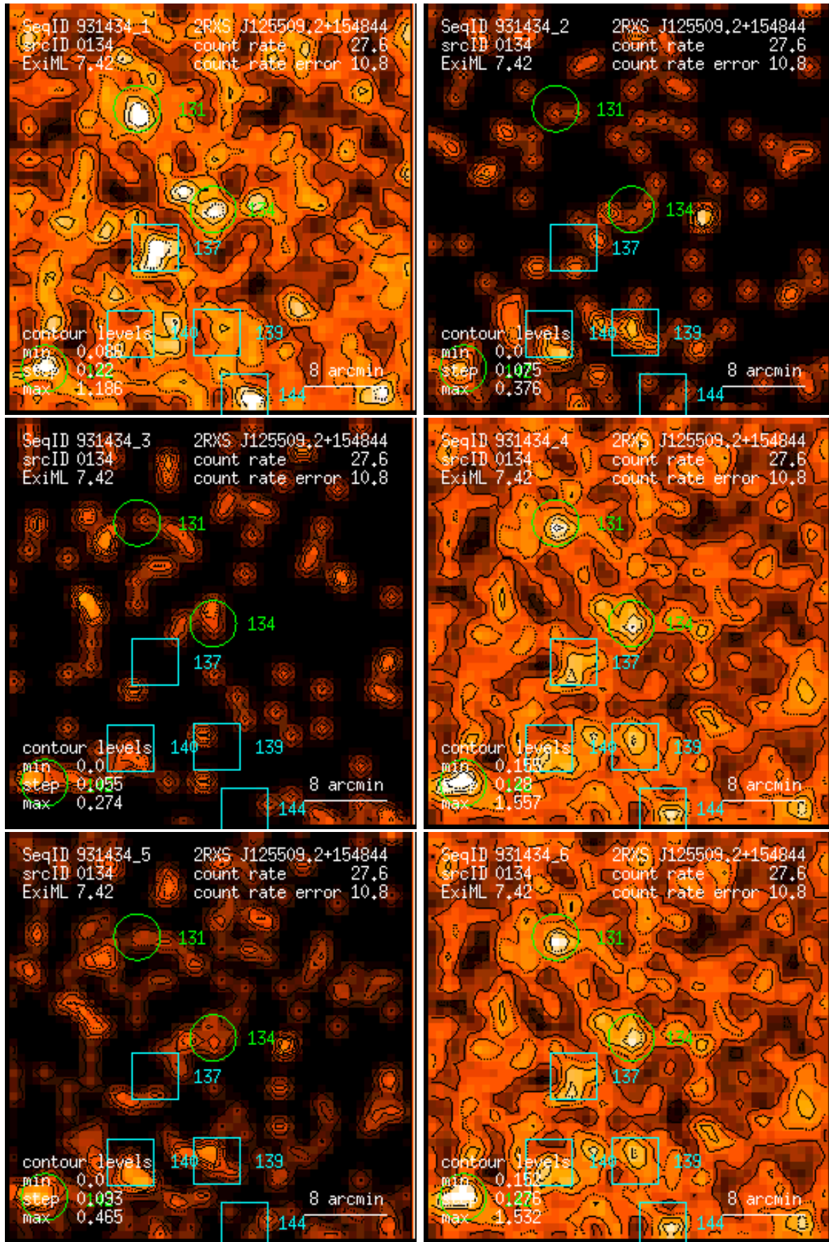
Figure 134: RASS 931434: detection 0134: band rate images, Gaussian filter: (1) PSPC channels 11 – 41, (2) 52 – 90, (3) 91 – 201, (4) 11 – 235, (5) 52 – 201, (6) 11 – 201. Broad band rates in counts/ks. Band rate contour levels in counts/ks/arcmin 2 .
