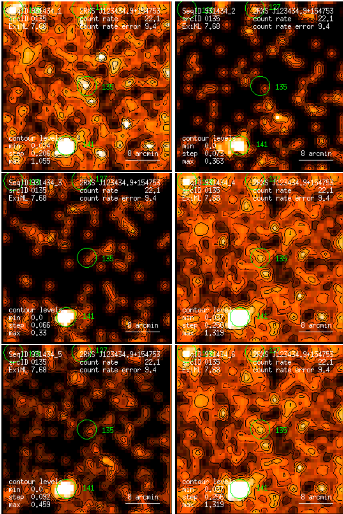
Figure 135: RASS 931434: detection 0135: band rate images, Gaussian filter: (1) PSPC channels 11 – 41, (2) 52 – 90, (3) 91 – 201, (4) 11 – 235, (5) 52 – 201, (6) 11 – 201. Broad band rates in counts/ks. Band rate contour levels in counts/ks/arcmin 2 .
