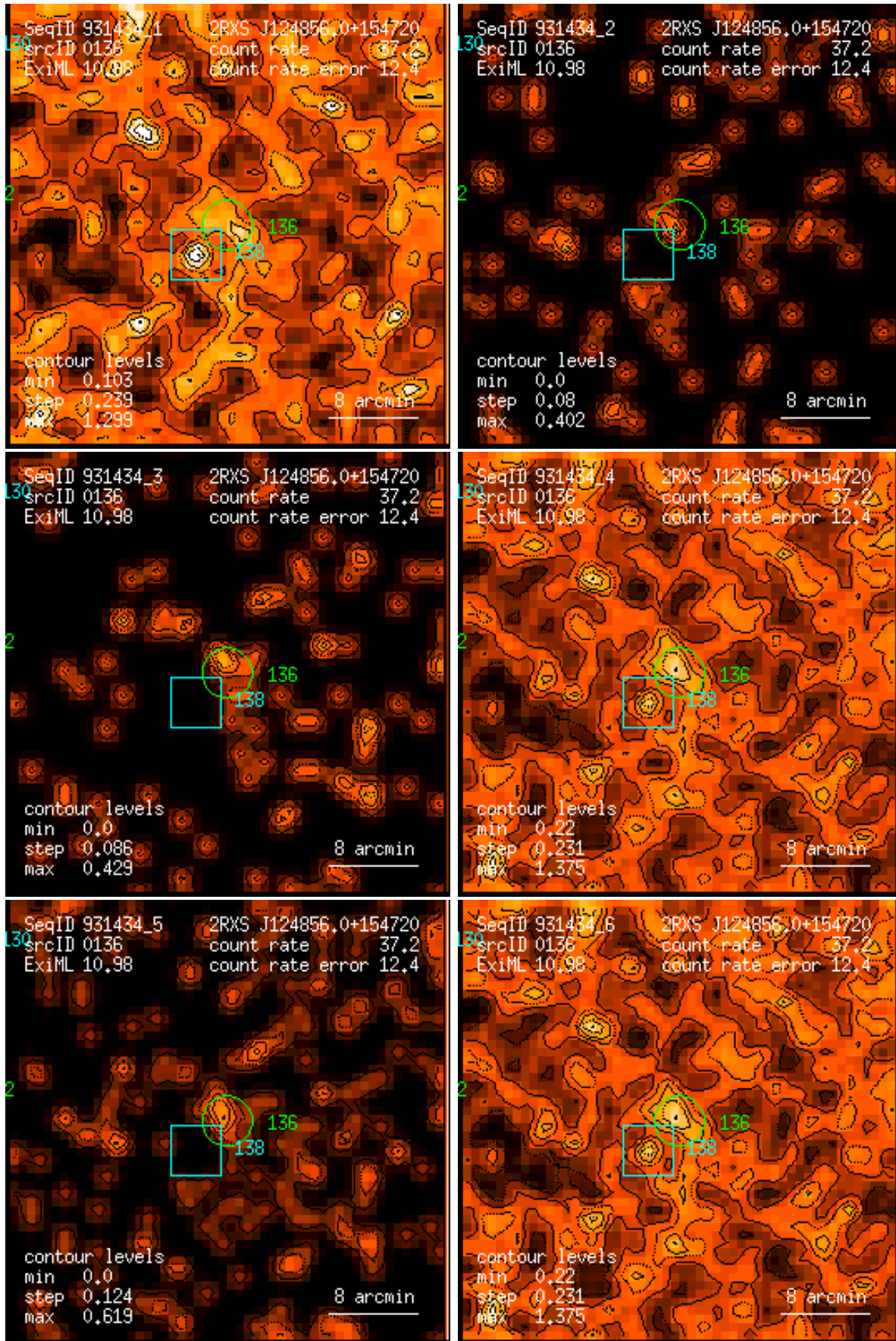
Figure 136: RASS 931434: detection 0136: band rate images, Gaussian filter: (1) PSPC channels 11 – 41, (2) 52 – 90, (3) 91 – 201, (4) 11 – 235, (5) 52 – 201, (6) 11 – 201. Broad band rates in counts/ks. Band rate contour levels in counts/ks/arcmin 2 .
