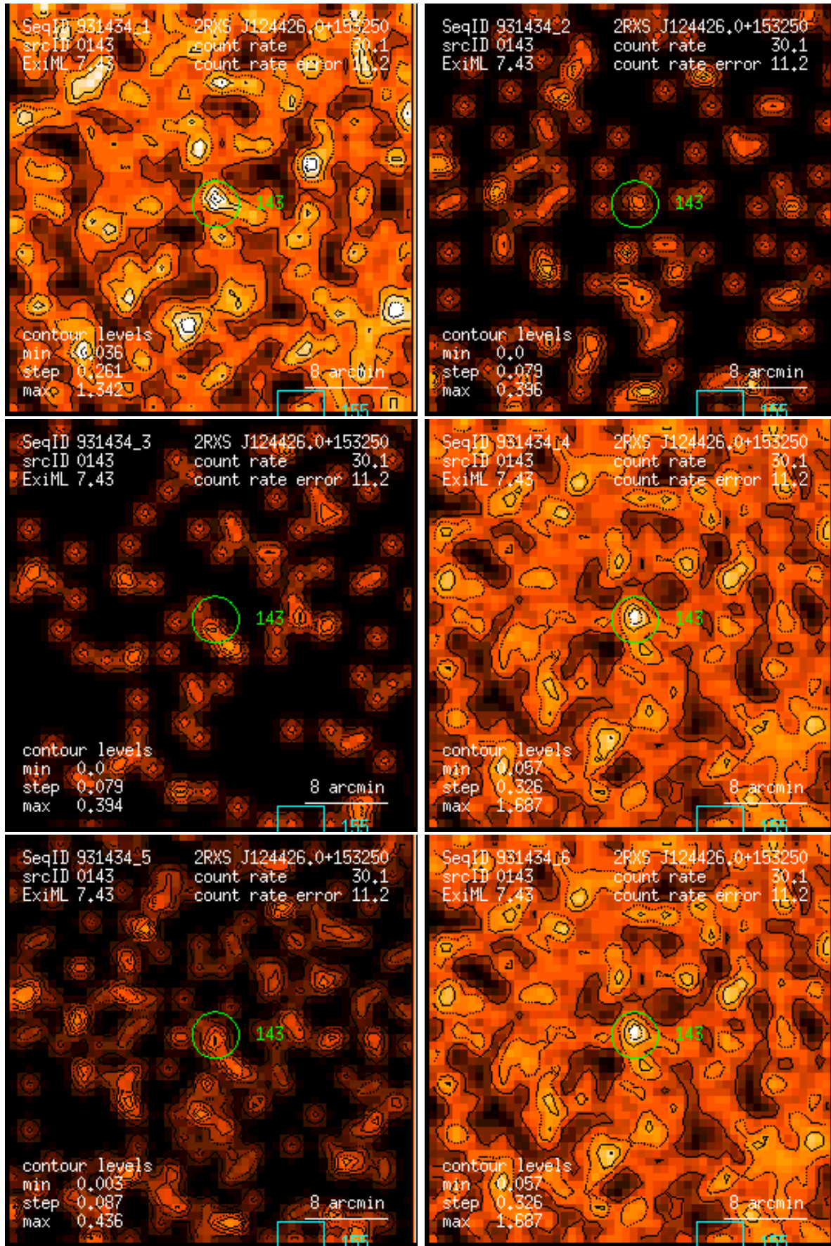
Figure 143: RASS 931434: detection 0143: band rate images, Gaussian filter: (1) PSPC channels 11 – 41, (2) 52 – 90, (3) 91 – 201, (4) 11 – 235, (5) 52 – 201, (6) 11 – 201. Broad band rates in counts/ks. Band rate contour levels in counts/ks/arcmin 2 .
