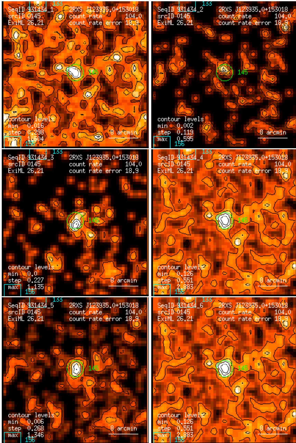
Figure 145: RASS 931434: detection 0145: band rate images, Gaussian filter: (1) PSPC channels 11 – 41, (2) 52 – 90, (3) 91 – 201, (4) 11 – 235, (5) 52 – 201, (6) 11 – 201. Broad band rates in counts/ks. Band rate contour levels in counts/ks/arcmin 2 .
