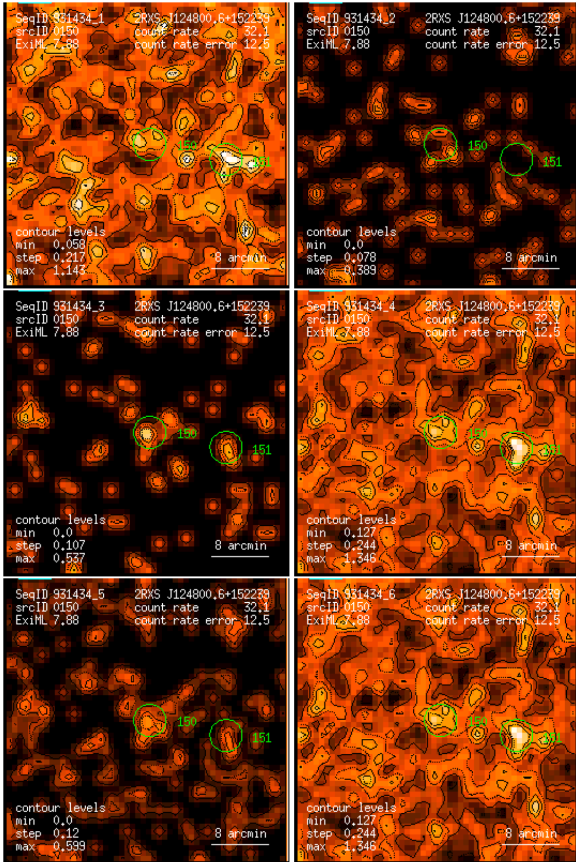
Figure 150: RASS 931434: detection 0150: band rate images, Gaussian filter: (1) PSPC channels 11 – 41, (2) 52 – 90, (3) 91 – 201, (4) 11 – 235, (5) 52 – 201, (6) 11 – 201. Broad band rates in counts/ks. Band rate contour levels in counts/ks/arcmin 2 .
