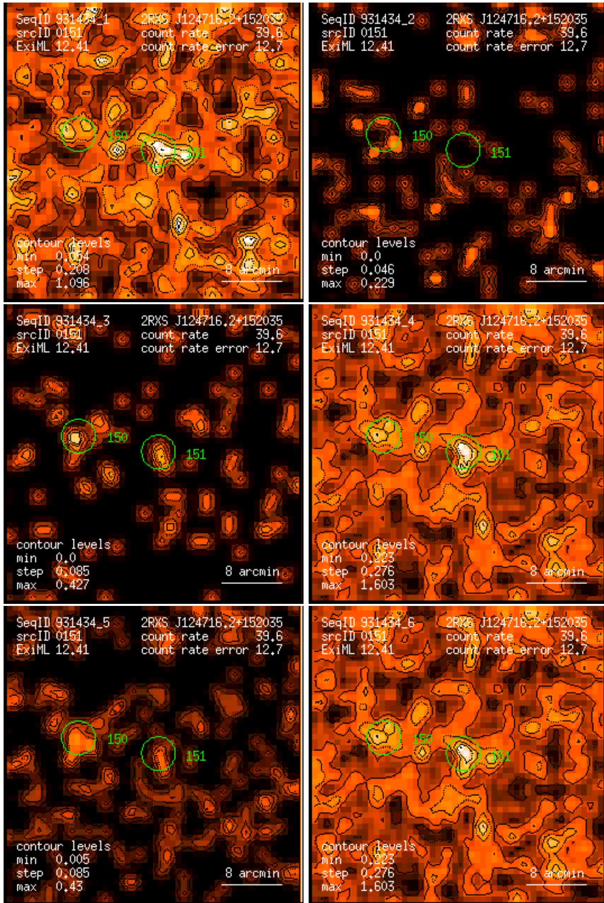
Figure 151: RASS 931434: detection 0151: band rate images, Gaussian filter: (1) PSPC channels 11 – 41, (2) 52 – 90, (3) 91 – 201, (4) 11 – 235, (5) 52 – 201, (6) 11 – 201. Broad band rates in counts/ks. Band rate contour levels in counts/ks/arcmin 2 .
