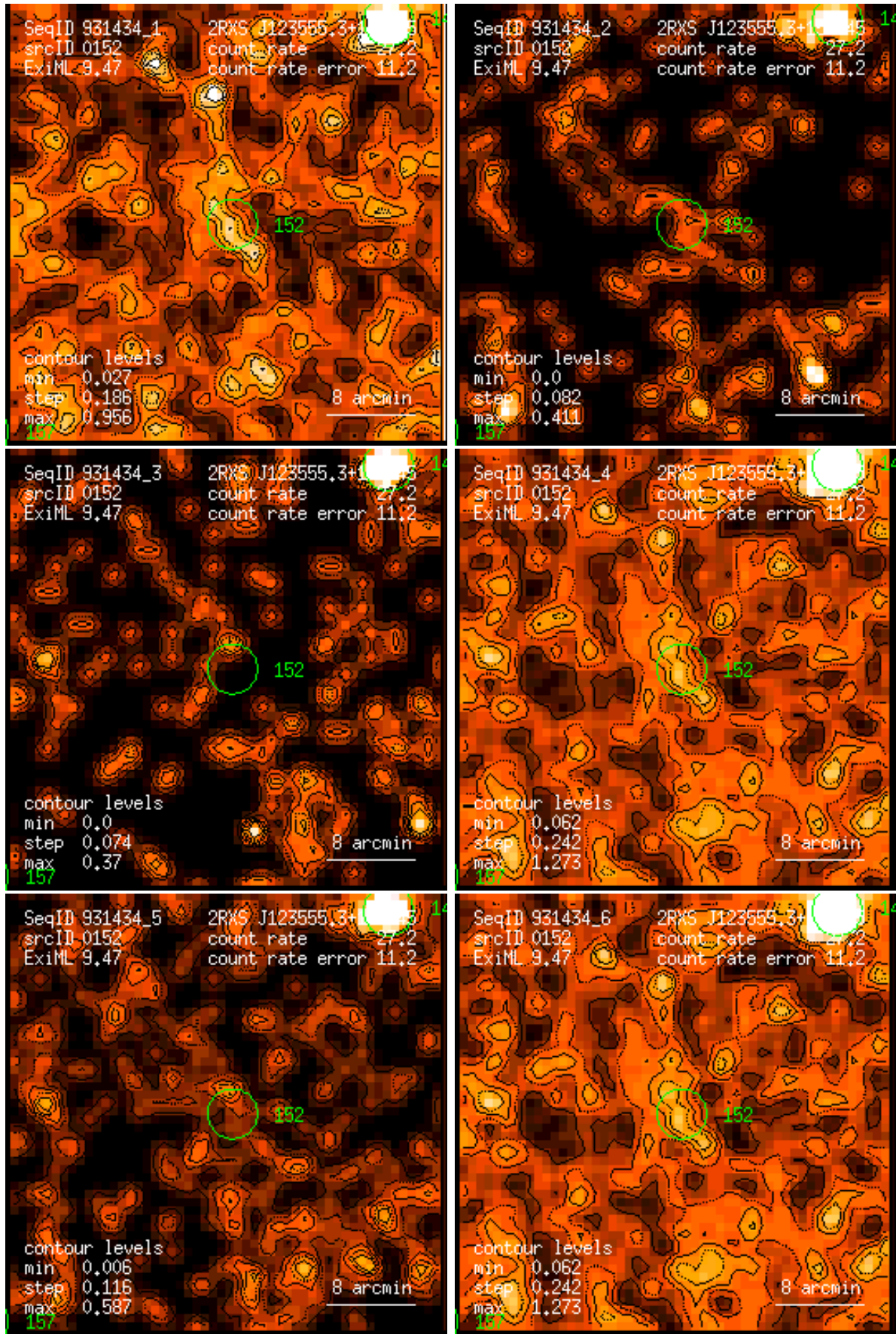
Figure 152: RASS 931434: detection 0152: band rate images, Gaussian filter: (1) PSPC channels 11 – 41, (2) 52 – 90, (3) 91 – 201, (4) 11 – 235, (5) 52 – 201, (6) 11 – 201. Broad band rates in counts/ks. Band rate contour levels in counts/ks/arcmin 2 .
