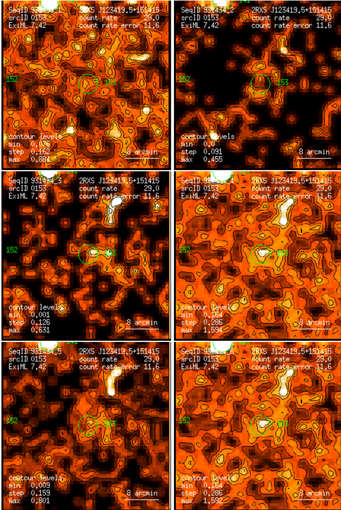
Figure 153: RASS 931434: detection 0153: band rate images, Gaussian filter: (1) PSPC channels 11 – 41, (2) 52 – 90, (3) 91 – 201, (4) 11 – 235, (5) 52 – 201, (6) 11 – 201. Broad band rates in counts/ks. Band rate contour levels in counts/ks/arcmin 2 .
