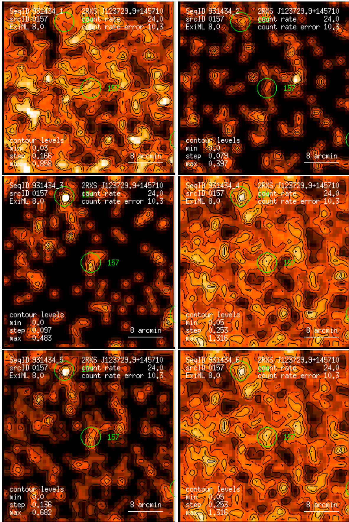
Figure 157: RASS 931434: detection 0157: band rate images, Gaussian filter: (1) PSPC channels 11 – 41, (2) 52 – 90, (3) 91 – 201, (4) 11 – 235, (5) 52 – 201, (6) 11 – 201. Broad band rates in counts/ks. Band rate contour levels in counts/ks/arcmin 2 .
