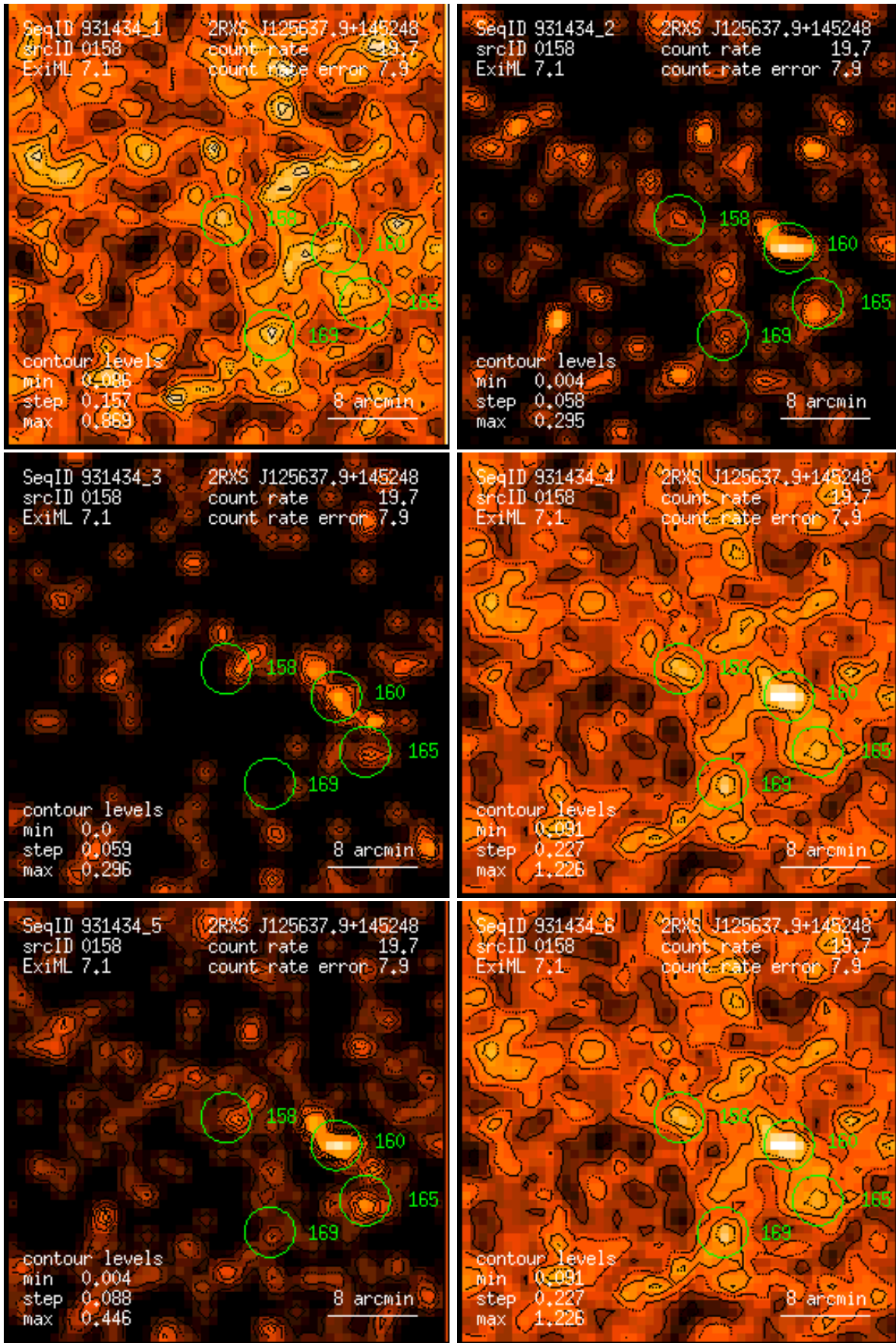
Figure 158: RASS 931434: detection 0158: band rate images, Gaussian filter: (1) PSPC channels 11 – 41, (2) 52 – 90, (3) 91 – 201, (4) 11 – 235, (5) 52 – 201, (6) 11 – 201. Broad band rates in counts/ks. Band rate contour levels in counts/ks/arcmin 2 .
