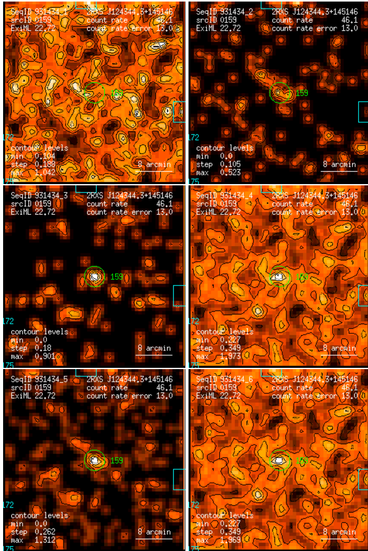
Figure 159: RASS 931434: detection 0159: band rate images, Gaussian filter: (1) PSPC channels 11 – 41, (2) 52 – 90, (3) 91 – 201, (4) 11 – 235, (5) 52 – 201, (6) 11 – 201. Broad band rates in counts/ks. Band rate contour levels in counts/ks/arcmin 2 .
