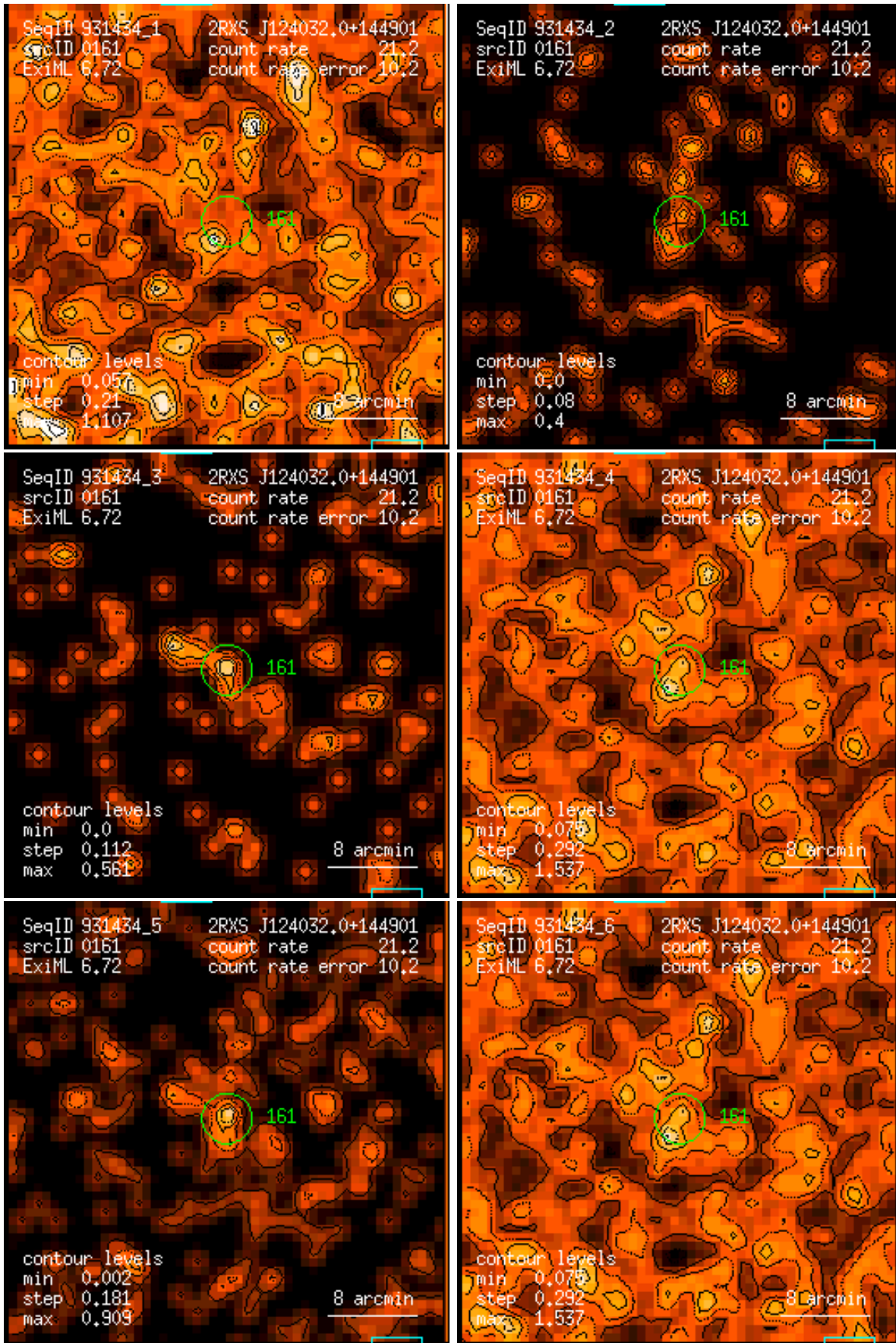
Figure 161: RASS 931434: detection 0161: band rate images, Gaussian filter: (1) PSPC channels 11 – 41, (2) 52 – 90, (3) 91 – 201, (4) 11 – 235, (5) 52 – 201, (6) 11 – 201. Broad band rates in counts/ks. Band rate contour levels in counts/ks/arcmin 2 .
