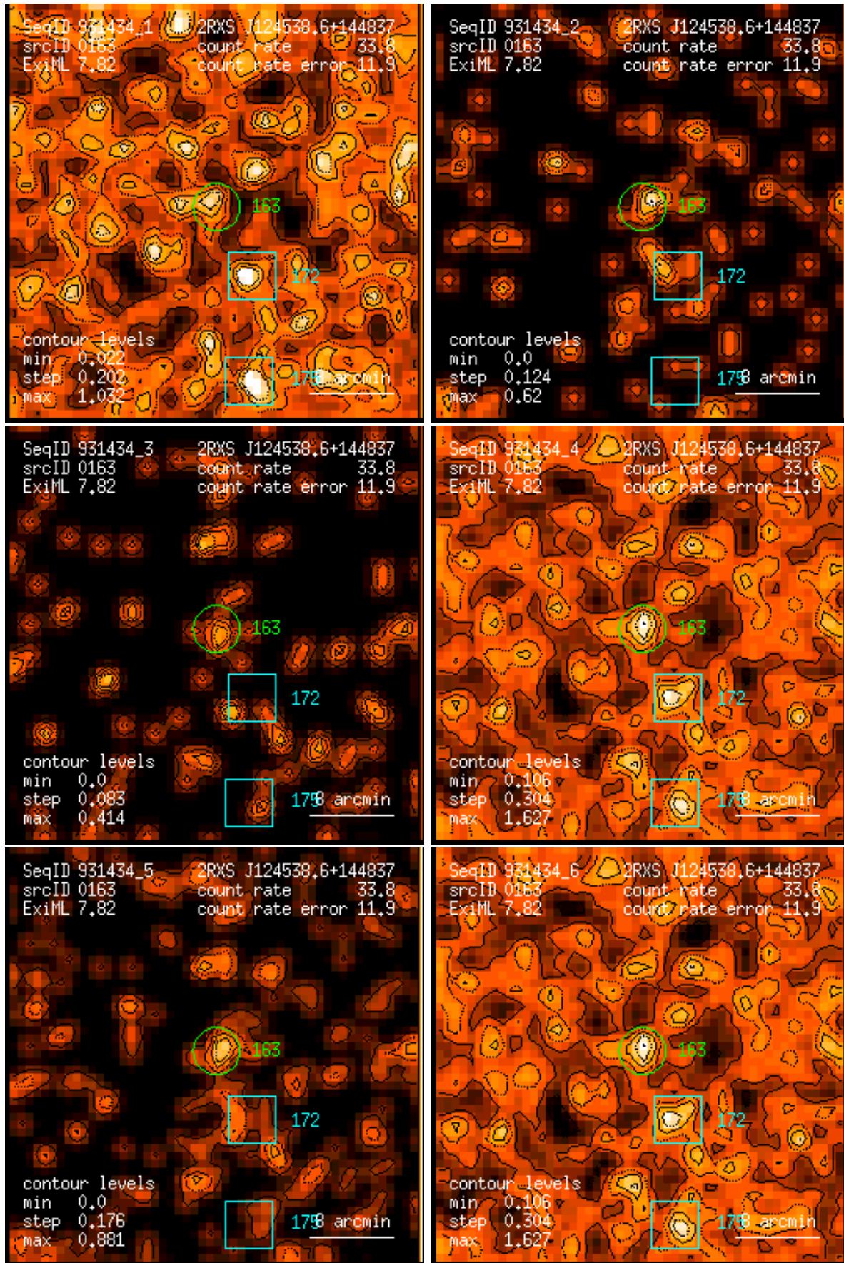
Figure 163: RASS 931434: detection 0163: band rate images, Gaussian filter: (1) PSPC channels 11 – 41, (2) 52 – 90, (3) 91 – 201, (4) 11 – 235, (5) 52 – 201, (6) 11 – 201. Broad band rates in counts/ks. Band rate contour levels in counts/ks/arcmin 2 .
