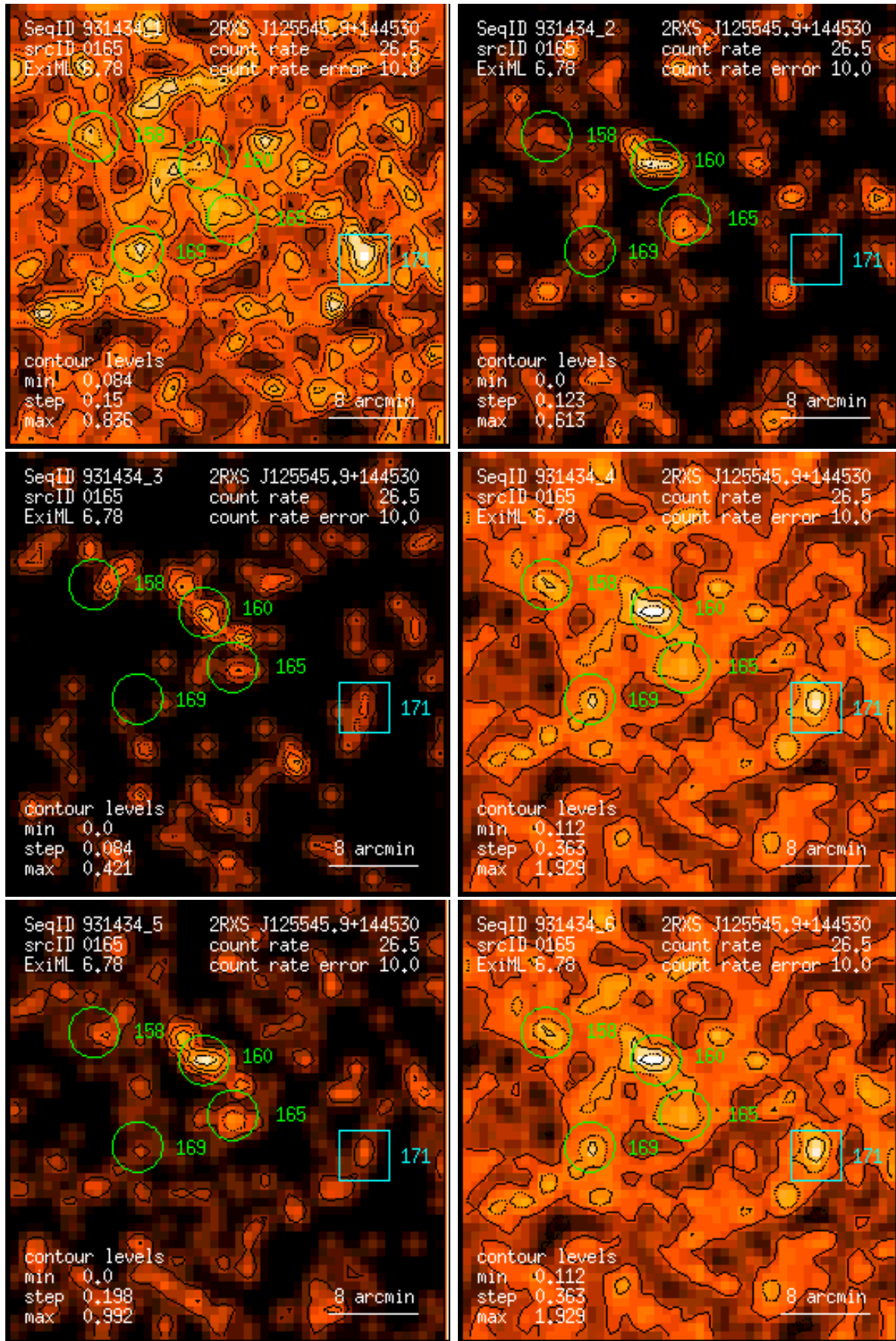
Figure 165: RASS 931434: detection 0165: band rate images, Gaussian filter: (1) PSPC channels 11 – 41, (2) 52 – 90, (3) 91 – 201, (4) 11 – 235, (5) 52 – 201, (6) 11 – 201. Broad band rates in counts/ks. Band rate contour levels in counts/ks/arcmin 2 .
