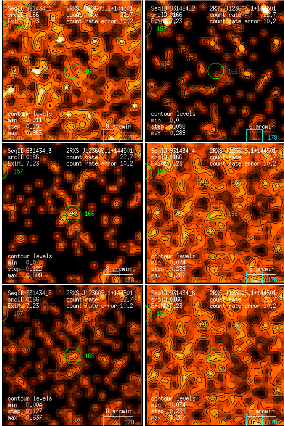
Figure 166: RASS 931434: detection 0166: band rate images, Gaussian filter: (1) PSPC channels 11 – 41, (2) 52 – 90, (3) 91 – 201, (4) 11 – 235, (5) 52 – 201, (6) 11 – 201. Broad band rates in counts/ks. Band rate contour levels in counts/ks/arcmin 2 .
