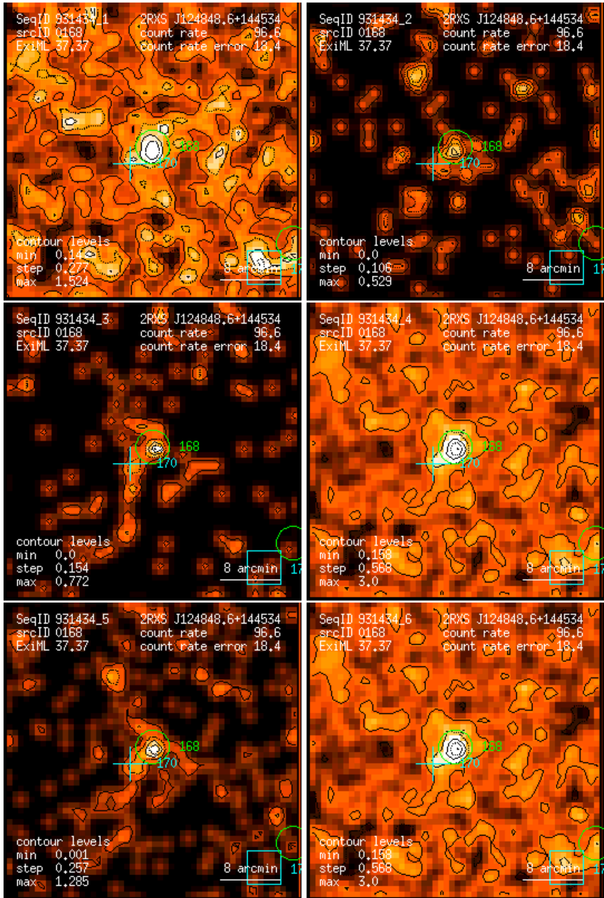
Figure 168: RASS 931434: detection 0168: band rate images, Gaussian filter: (1) PSPC channels 11 – 41, (2) 52 – 90, (3) 91 – 201, (4) 11 – 235, (5) 52 – 201, (6) 11 – 201. Broad band rates in counts/ks. Band rate contour levels in counts/ks/arcmin 2 .
