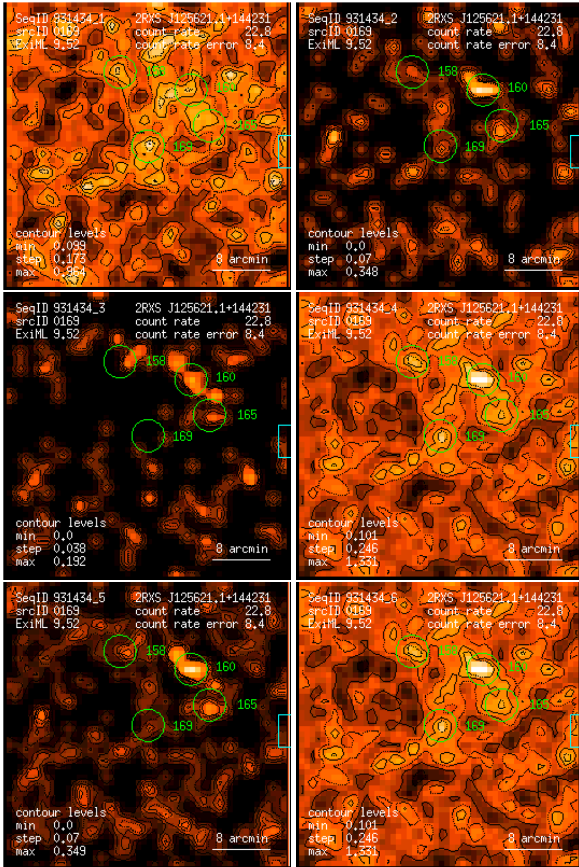
Figure 169: RASS 931434: detection 0169: band rate images, Gaussian filter: (1) PSPC channels 11 – 41, (2) 52 – 90, (3) 91 – 201, (4) 11 – 235, (5) 52 – 201, (6) 11 – 201. Broad band rates in counts/ks. Band rate contour levels in counts/ks/arcmin 2 .
