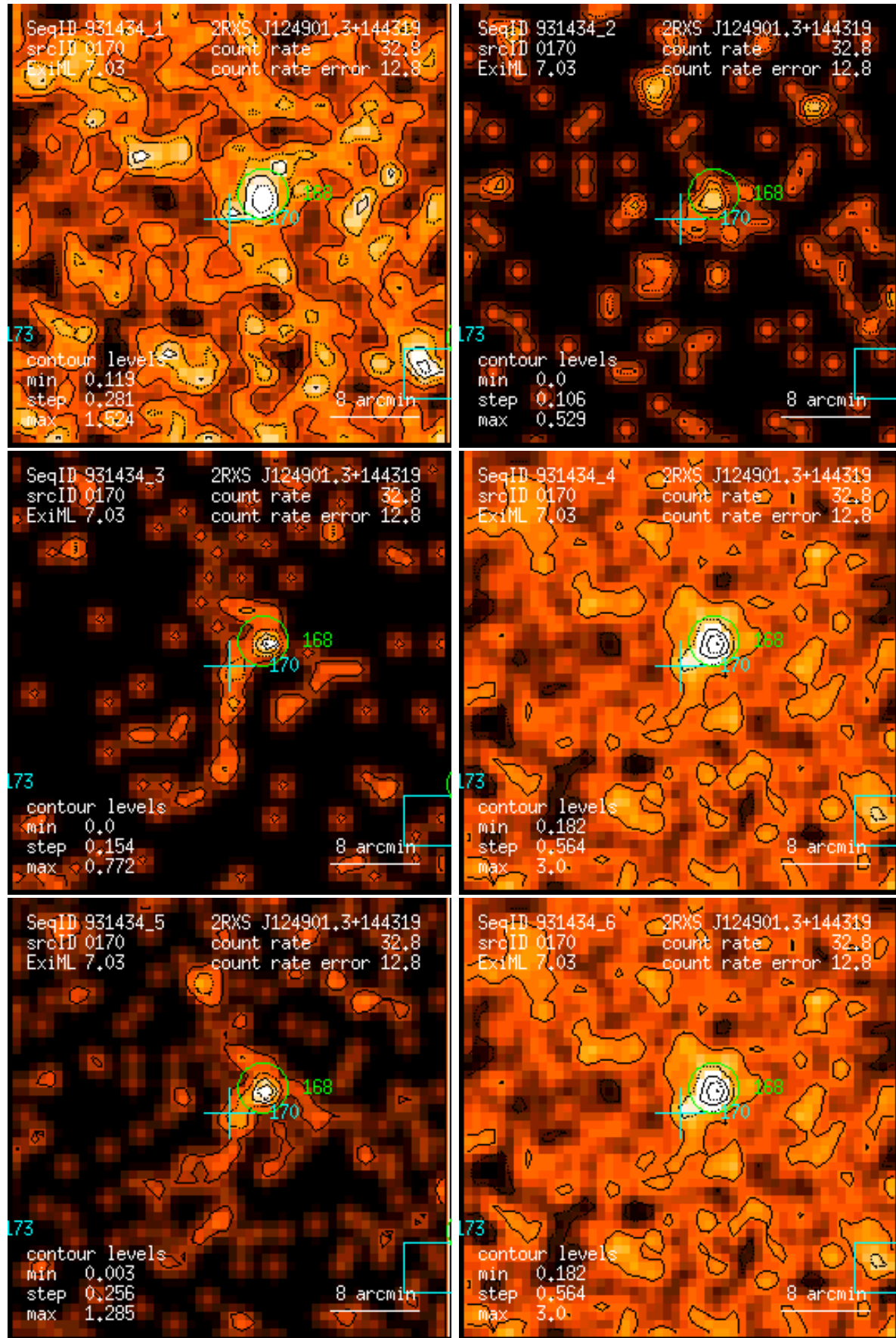
Figure 170: RASS 931434: detection 0170: band rate images, Gaussian filter: (1) PSPC channels 11 – 41, (2) 52 – 90, (3) 91 – 201, (4) 11 – 235, (5) 52 – 201, (6) 11 – 201. Broad band rates in counts/ks. Band rate contour levels in counts/ks/arcmin 2 .
