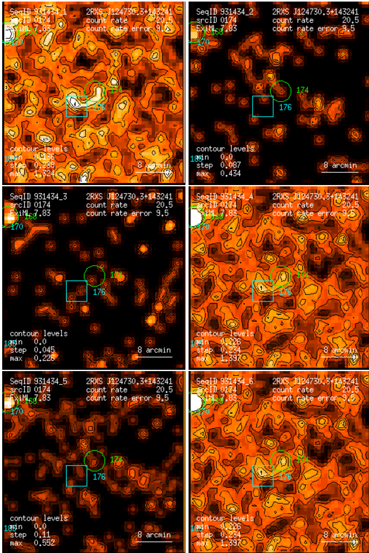
Figure 174: RASS 931434: detection 0174: band rate images, Gaussian filter: (1) PSPC channels 11 – 41, (2) 52 – 90, (3) 91 – 201, (4) 11 – 235, (5) 52 – 201, (6) 11 – 201. Broad band rates in counts/ks. Band rate contour levels in counts/ks/arcmin 2 .
