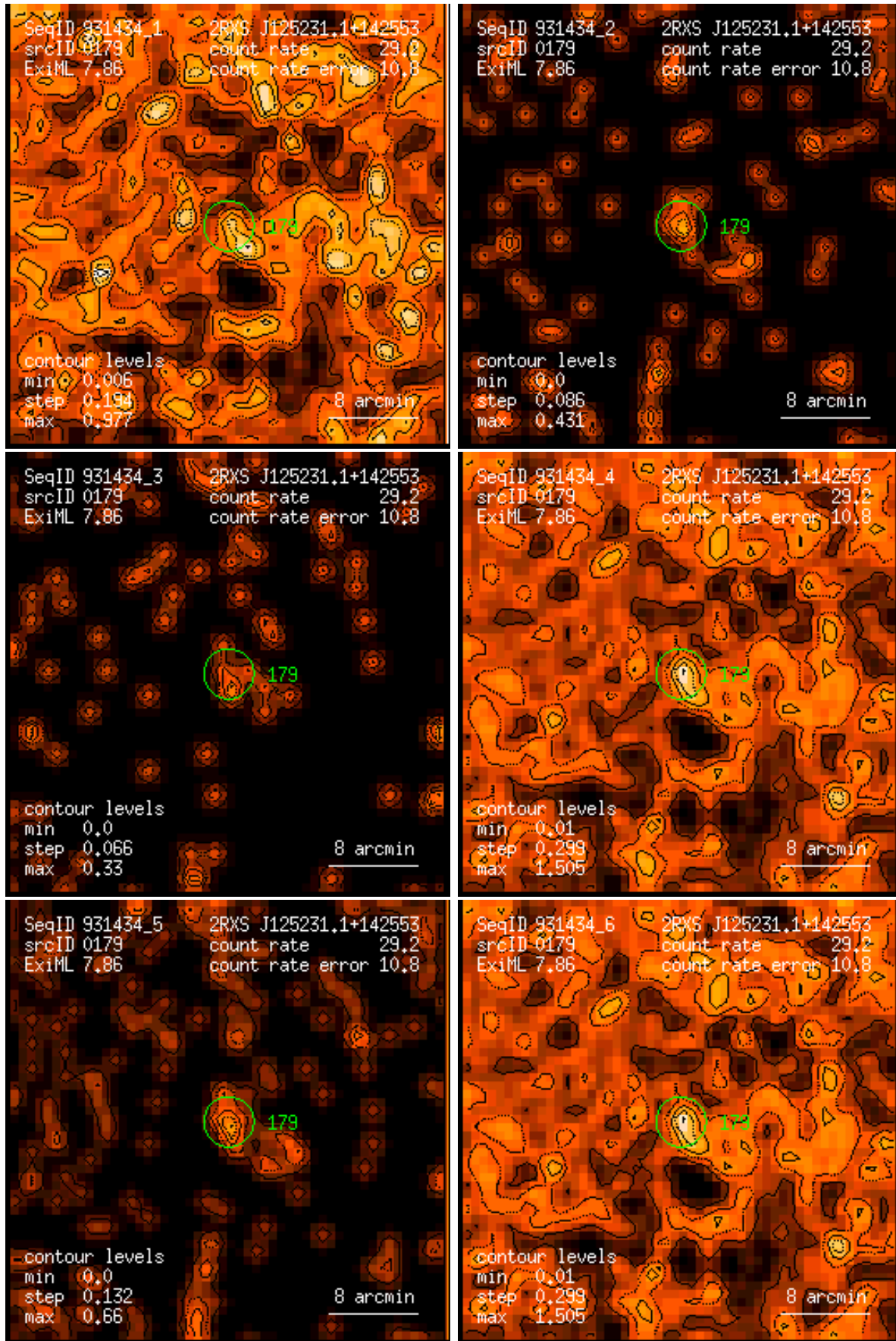
Figure 179: RASS 931434: detection 0179: band rate images, Gaussian filter: (1) PSPC channels 11 – 41, (2) 52 – 90, (3) 91 – 201, (4) 11 – 235, (5) 52 – 201, (6) 11 – 201. Broad band rates in counts/ks. Band rate contour levels in counts/ks/arcmin 2 .
