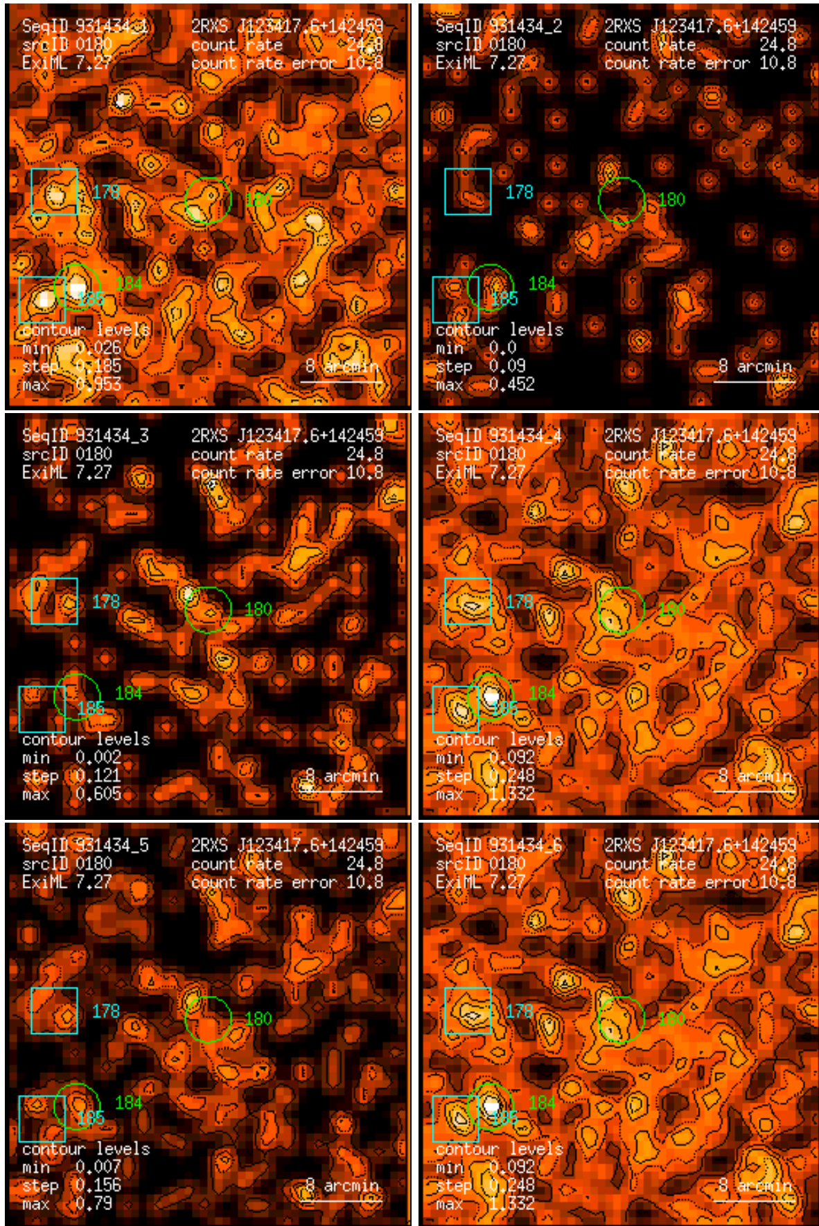
Figure 180: RASS 931434: detection 0180: band rate images, Gaussian filter: (1) PSPC channels 11 – 41, (2) 52 – 90, (3) 91 – 201, (4) 11 – 235, (5) 52 – 201, (6) 11 – 201. Broad band rates in counts/ks. Band rate contour levels in counts/ks/arcmin 2 .
