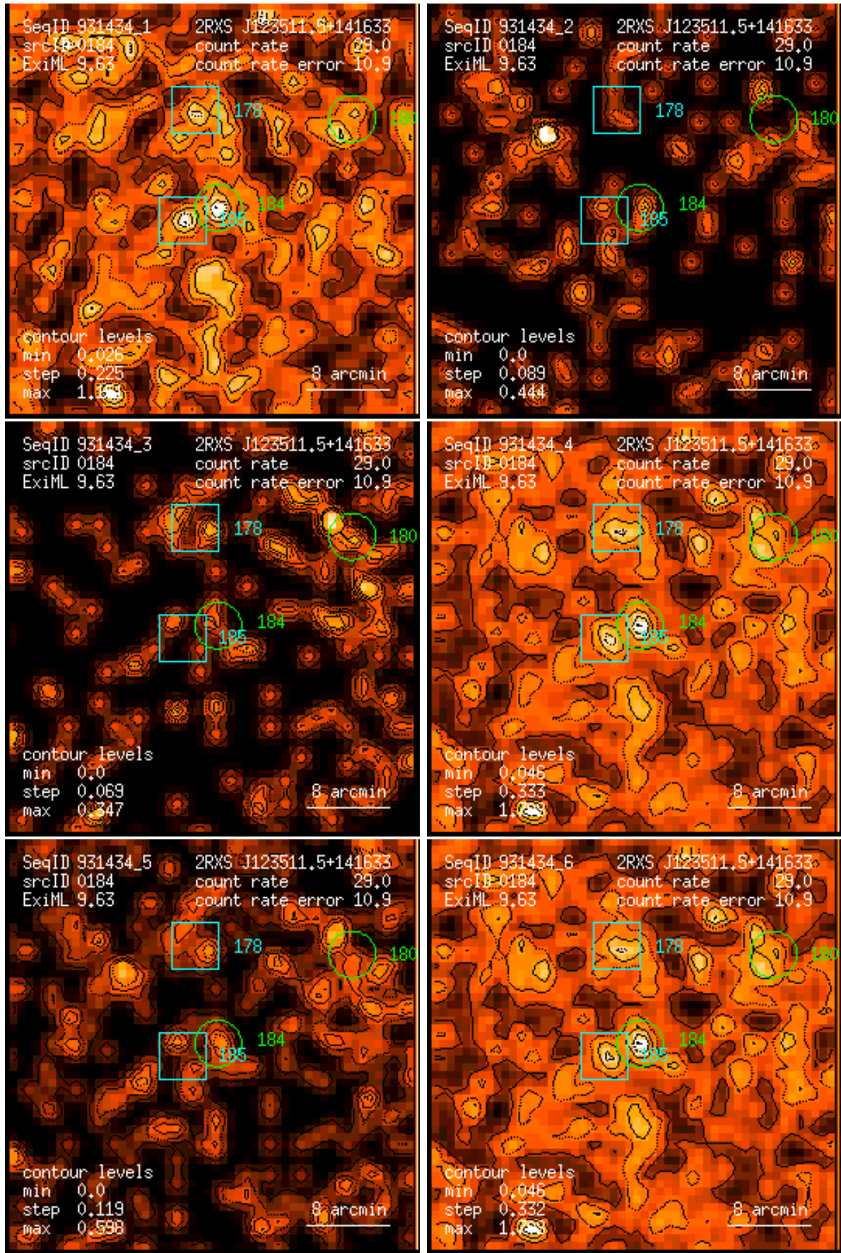
Figure 184: RASS 931434: detection 0184: band rate images, Gaussian filter: (1) PSPC channels 11 – 41, (2) 52 – 90, (3) 91 – 201, (4) 11 – 235, (5) 52 – 201, (6) 11 – 201. Broad band rates in counts/ks. Band rate contour levels in counts/ks/arcmin 2 .
