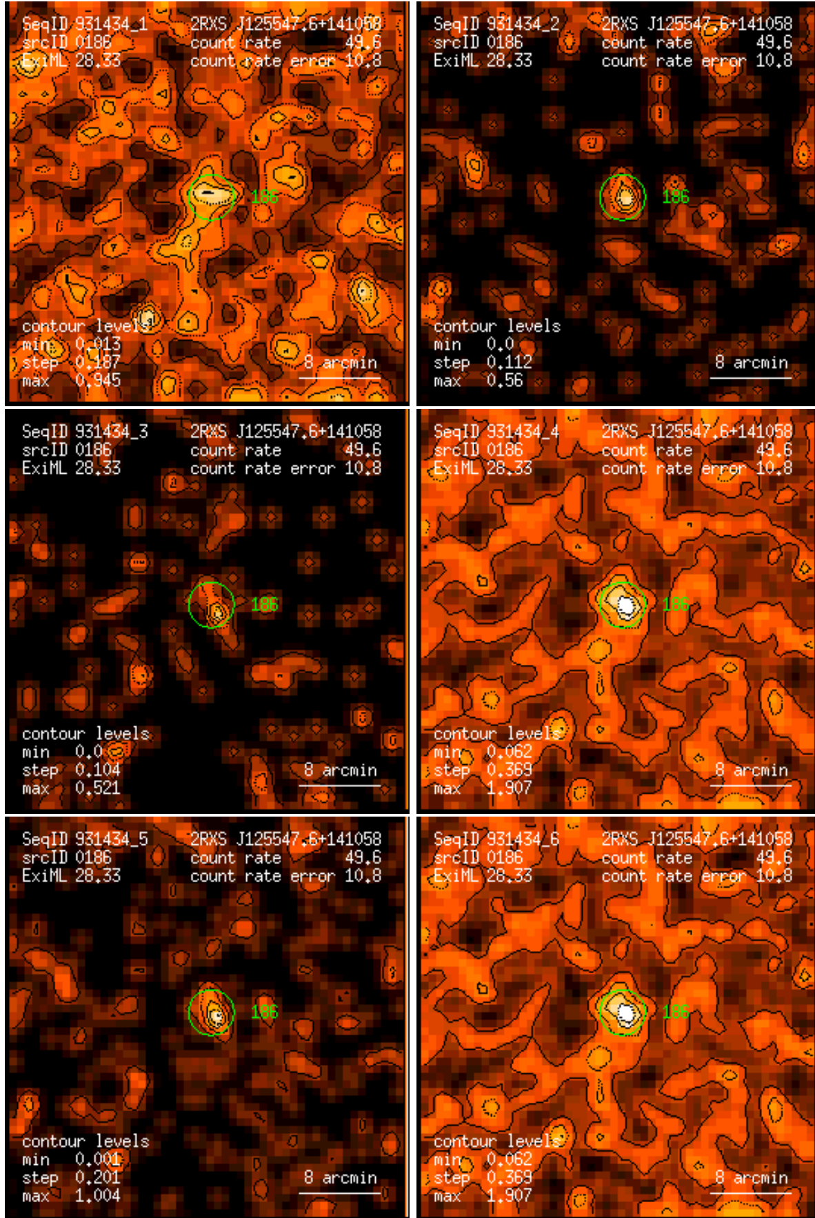
Figure 186: RASS 931434: detection 0186: band rate images, Gaussian filter: (1) PSPC channels 11 – 41, (2) 52 – 90, (3) 91 – 201, (4) 11 – 235, (5) 52 – 201, (6) 11 – 201. Broad band rates in counts/ks. Band rate contour levels in counts/ks/arcmin 2 .
