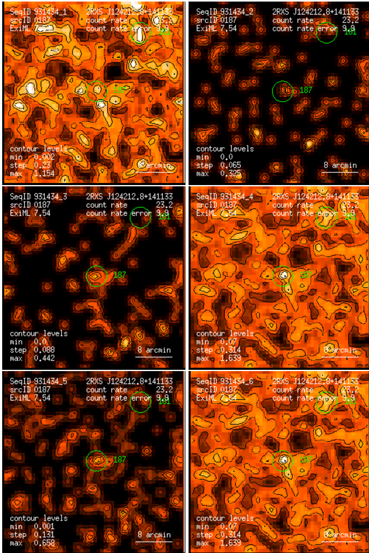
Figure 187: RASS 931434: detection 0187: band rate images, Gaussian filter: (1) PSPC channels 11 – 41, (2) 52 – 90, (3) 91 – 201, (4) 11 – 235, (5) 52 – 201, (6) 11 – 201. Broad band rates in counts/ks. Band rate contour levels in counts/ks/arcmin 2 .
