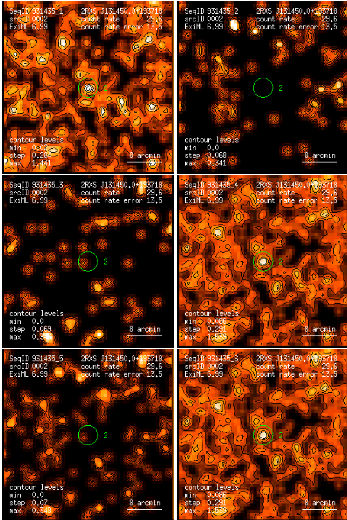
Figure 2: RASS 931435: detection 0002: band rate images, Gaussian filter: (1) PSPC channels 11 – 41, (2) 52 – 90, (3) 91 – 201, (4) 11 – 235, (5) 52 – 201, (6) 11 – 201. Broad band rates in counts/ks. Band rate contour levels in counts/ks/arcmin 2 .
