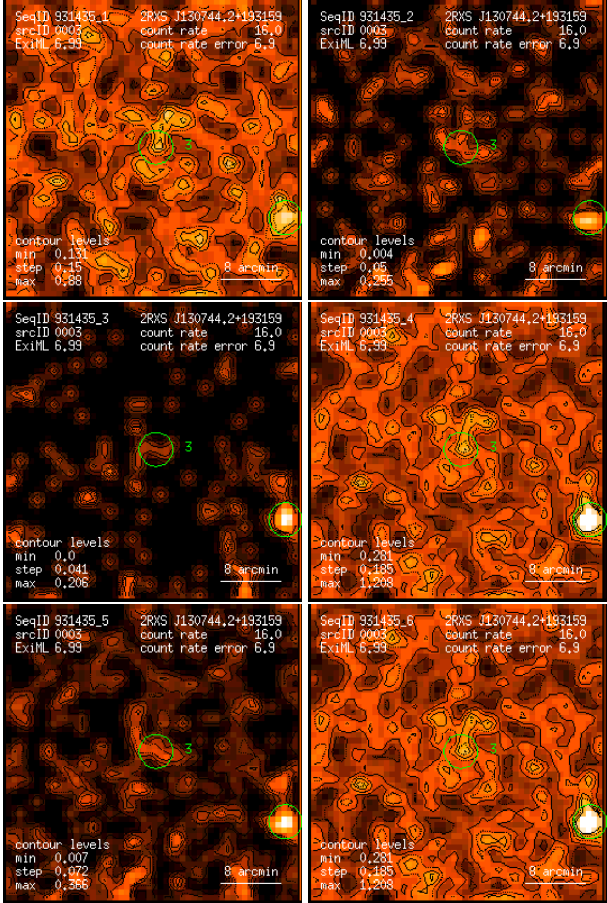
Figure 3: RASS 931435: detection 0003: band rate images, Gaussian filter: (1) PSPC channels 11 – 41, (2) 52 – 90, (3) 91 – 201, (4) 11 – 235, (5) 52 – 201, (6) 11 – 201. Broad band rates in counts/ks. Band rate contour levels in counts/ks/arcmin 2 .
