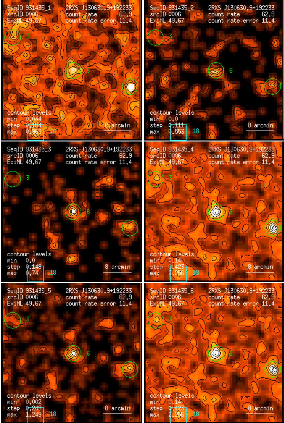
Figure 6: RASS 931435: detection 0006: band rate images, Gaussian filter: (1) PSPC channels 11 – 41, (2) 52 – 90, (3) 91 – 201, (4) 11 – 235, (5) 52 – 201, (6) 11 – 201. Broad band rates in counts/ks. Band rate contour levels in counts/ks/arcmin 2 .
