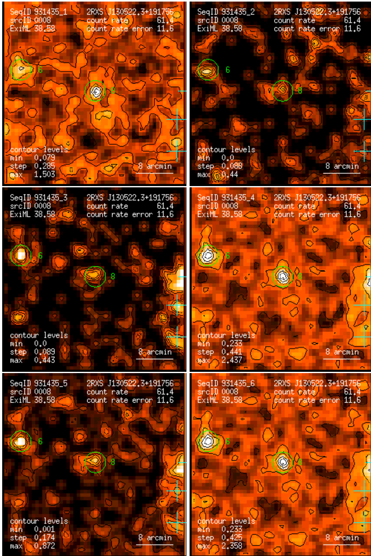
Figure 8: RASS 931435: detection 0008: band rate images, Gaussian filter: (1) PSPC channels 11 – 41, (2) 52 – 90, (3) 91 – 201, (4) 11 – 235, (5) 52 – 201, (6) 11 – 201. Broad band rates in counts/ks. Band rate contour levels in counts/ks/arcmin 2 .
