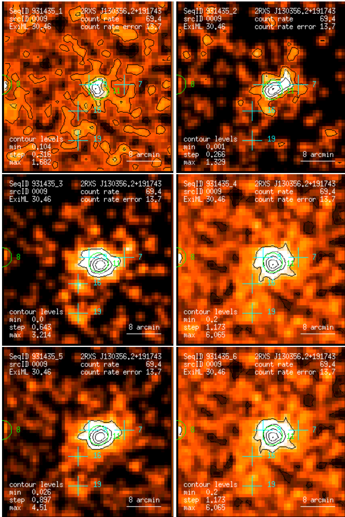
Figure 9: RASS 931435: detection 0009: band rate images, Gaussian filter: (1) PSPC channels 11 – 41, (2) 52 – 90, (3) 91 – 201, (4) 11 – 235, (5) 52 – 201, (6) 11 – 201. Broad band rates in counts/ks. Band rate contour levels in counts/ks/arcmin 2 .
