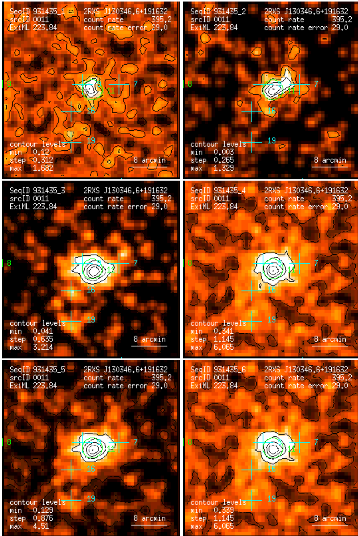
Figure 11: RASS 931435: detection 0011: band rate images, Gaussian filter: (1) PSPC channels 11 – 41, (2) 52 – 90, (3) 91 – 201, (4) 11 – 235, (5) 52 – 201, (6) 11 – 201. Broad band rates in counts/ks. Band rate contour levels in counts/ks/arcmin 2 .
