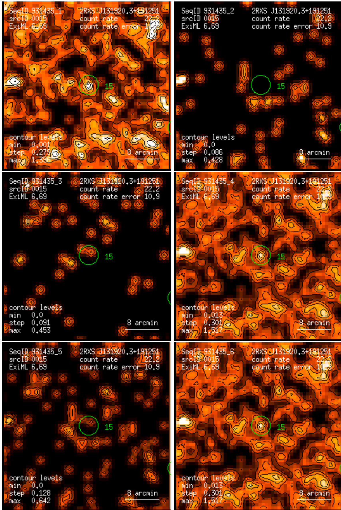
Figure 15: RASS 931435: detection 0015: band rate images, Gaussian filter: (1) PSPC channels 11 – 41, (2) 52 – 90, (3) 91 – 201, (4) 11 – 235, (5) 52 – 201, (6) 11 – 201. Broad band rates in counts/ks. Band rate contour levels in counts/ks/arcmin 2 .
