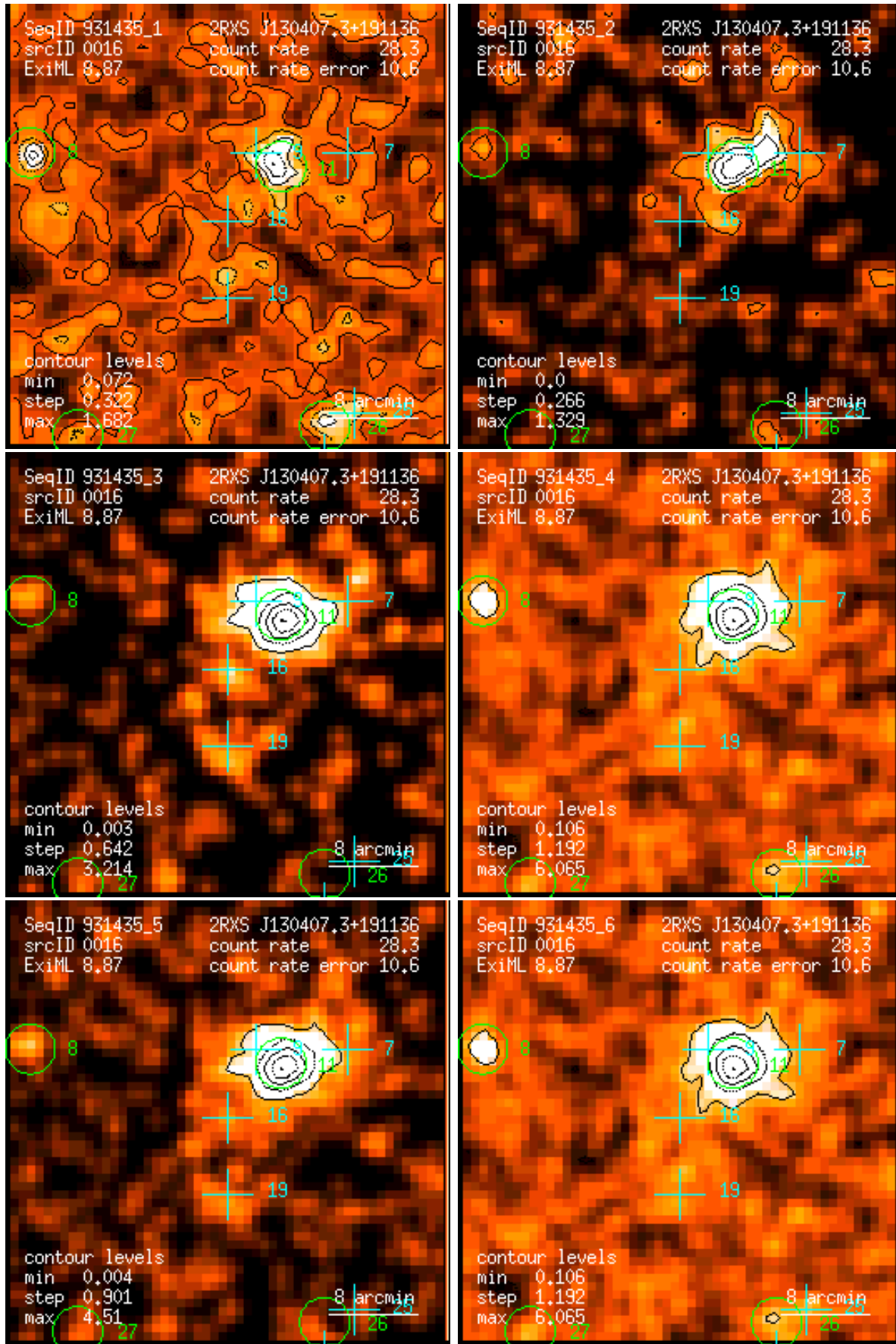
Figure 16: RASS 931435: detection 0016: band rate images, Gaussian filter: (1) PSPC channels 11 – 41, (2) 52 – 90, (3) 91 – 201, (4) 11 – 235, (5) 52 – 201, (6) 11 – 201. Broad band rates in counts/ks. Band rate contour levels in counts/ks/arcmin 2 .
