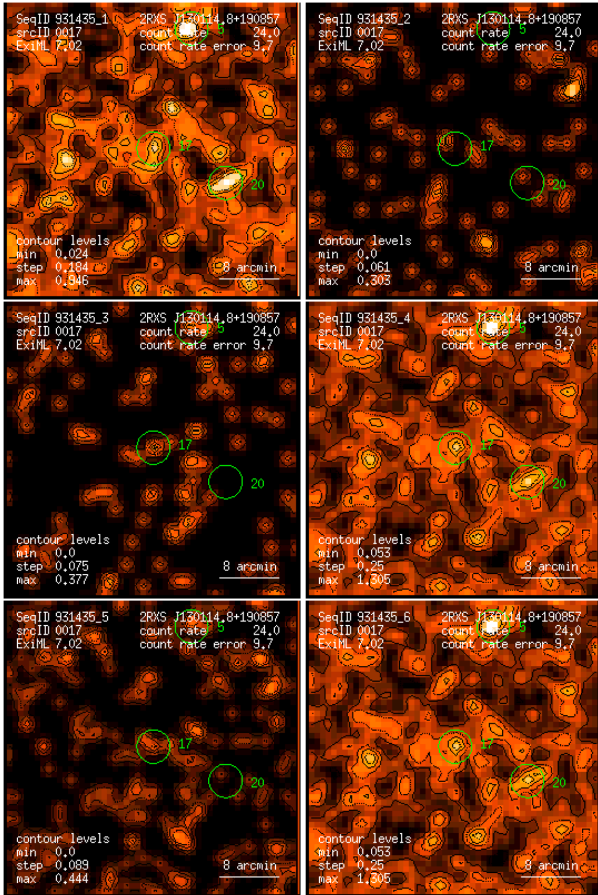
Figure 17: RASS 931435: detection 0017: band rate images, Gaussian filter: (1) PSPC channels 11 – 41, (2) 52 – 90, (3) 91 – 201, (4) 11 – 235, (5) 52 – 201, (6) 11 – 201. Broad band rates in counts/ks. Band rate contour levels in counts/ks/arcmin 2 .
