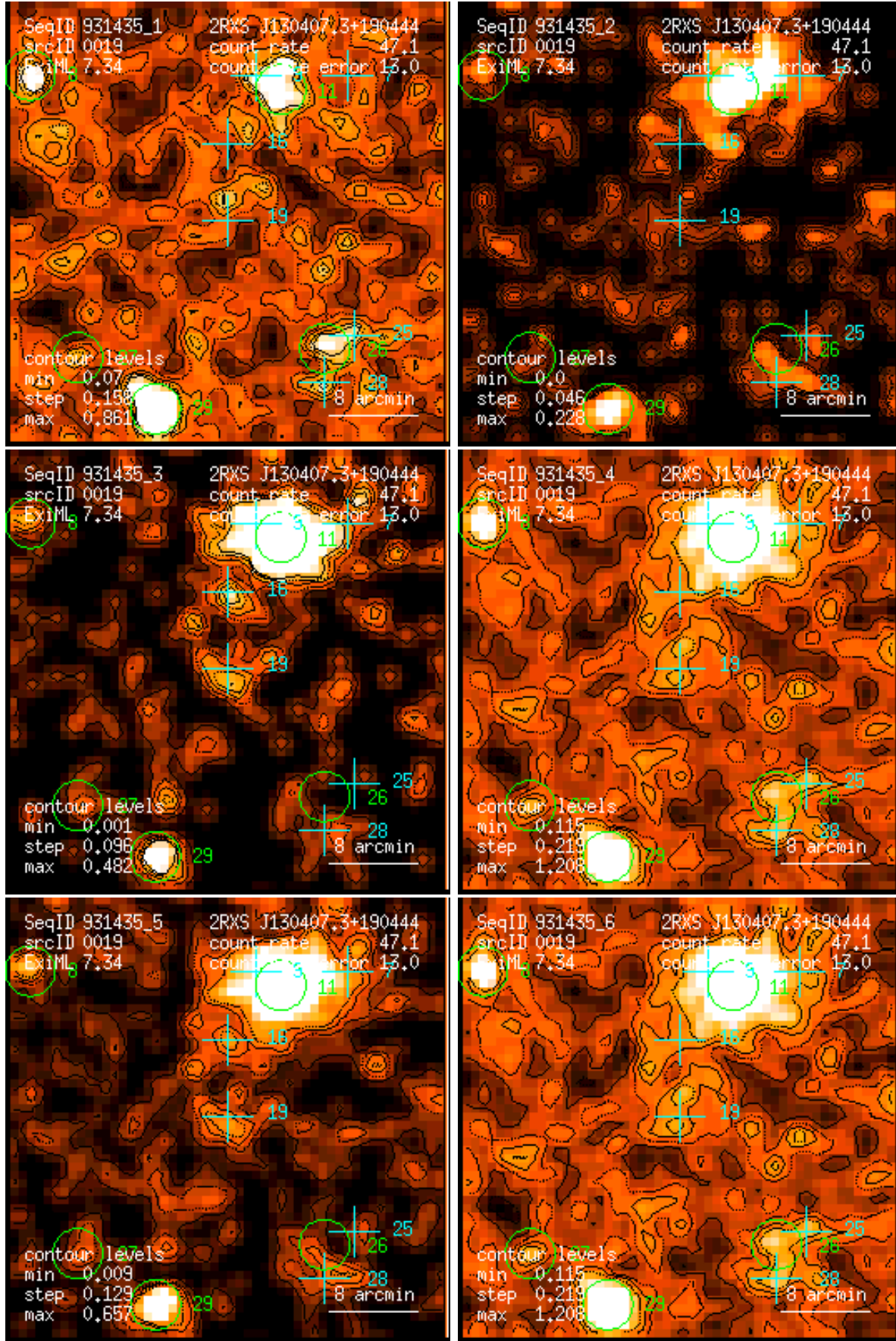
Figure 19: RASS 931435: detection 0019: band rate images, Gaussian filter: (1) PSPC channels 11 – 41, (2) 52 – 90, (3) 91 – 201, (4) 11 – 235, (5) 52 – 201, (6) 11 – 201. Broad band rates in counts/ks. Band rate contour levels in counts/ks/arcmin 2 .
