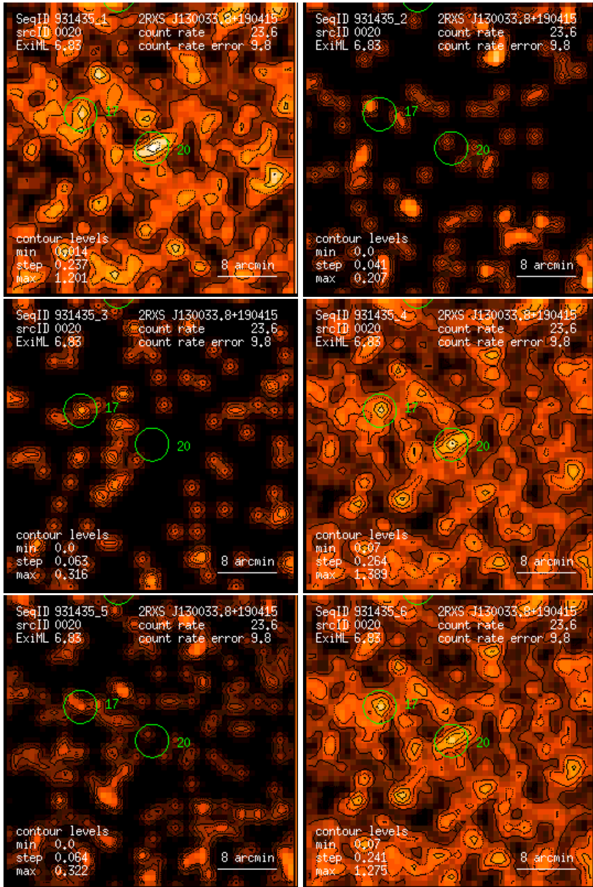
Figure 20: RASS 931435: detection 0020: band rate images, Gaussian filter: (1) PSPC channels 11 – 41, (2) 52 – 90, (3) 91 – 201, (4) 11 – 235, (5) 52 – 201, (6) 11 – 201. Broad band rates in counts/ks. Band rate contour levels in counts/ks/arcmin 2 .
