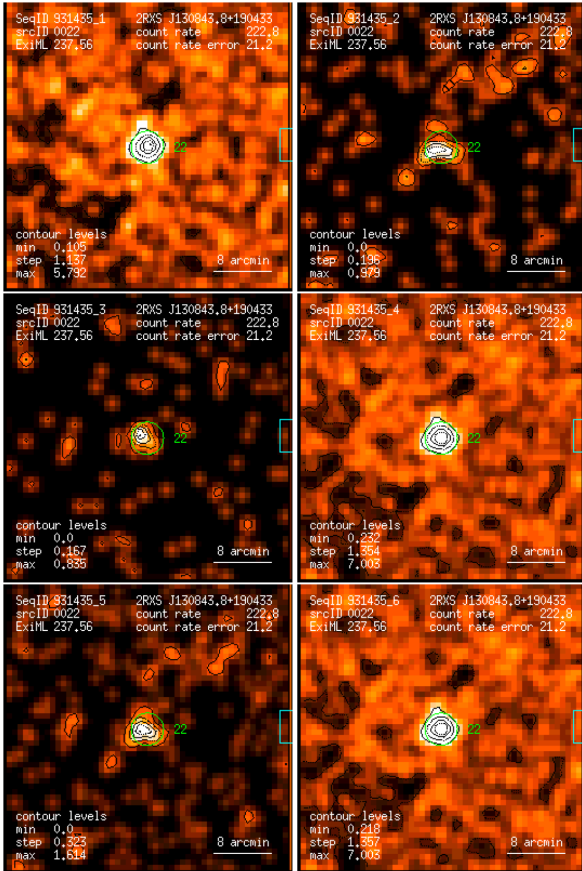
Figure 22: RASS 931435: detection 0022: band rate images, Gaussian filter: (1) PSPC channels 11 – 41, (2) 52 – 90, (3) 91 – 201, (4) 11 – 235, (5) 52 – 201, (6) 11 – 201. Broad band rates in counts/ks. Band rate contour levels in counts/ks/arcmin 2 .
