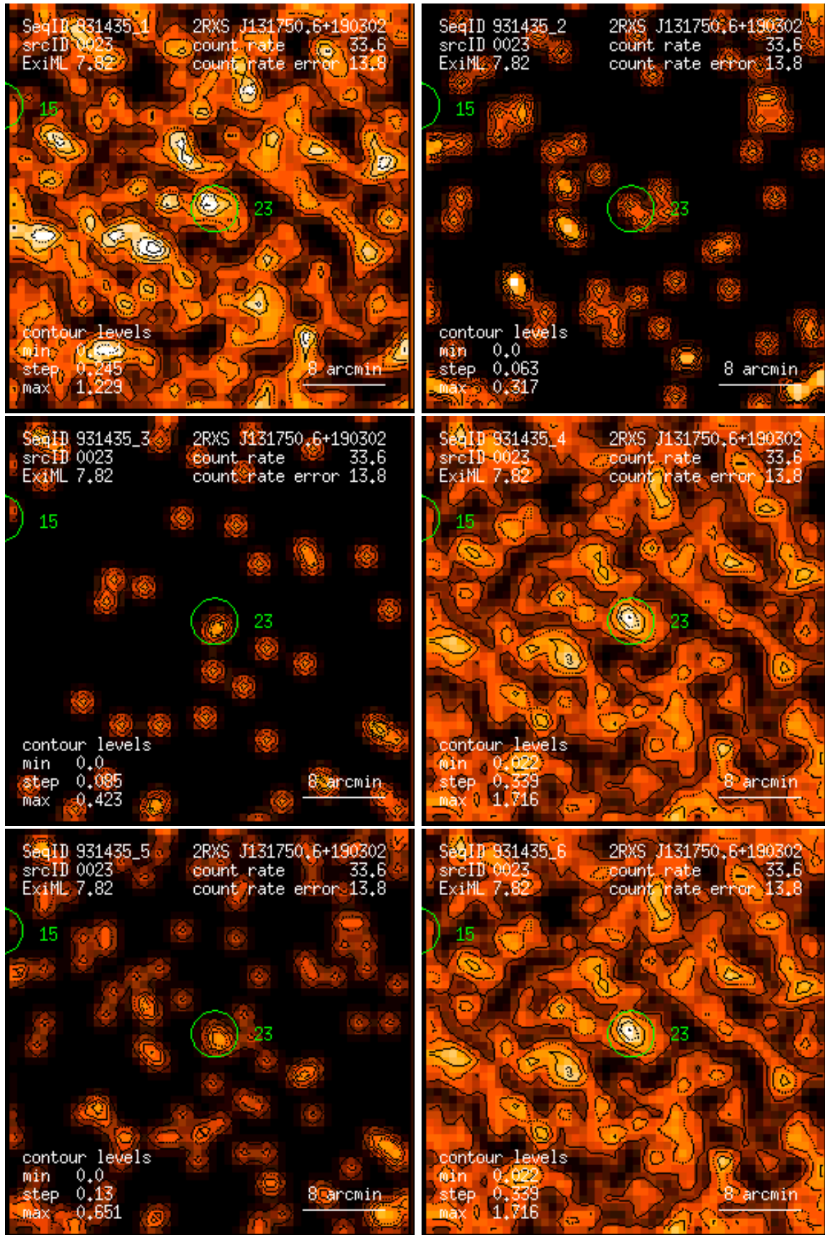
Figure 23: RASS 931435: detection 0023: band rate images, Gaussian filter: (1) PSPC channels 11 – 41, (2) 52 – 90, (3) 91 – 201, (4) 11 – 235, (5) 52 – 201, (6) 11 – 201. Broad band rates in counts/ks. Band rate contour levels in counts/ks/arcmin 2 .
