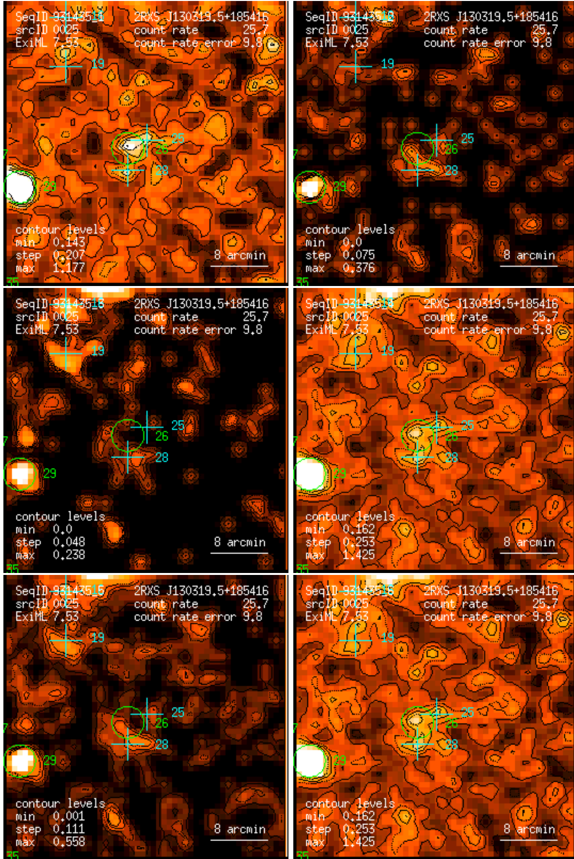
Figure 25: RASS 931435: detection 0025: band rate images, Gaussian filter: (1) PSPC channels 11 – 41, (2) 52 – 90, (3) 91 – 201, (4) 11 – 235, (5) 52 – 201, (6) 11 – 201. Broad band rates in counts/ks. Band rate contour levels in counts/ks/arcmin 2 .
