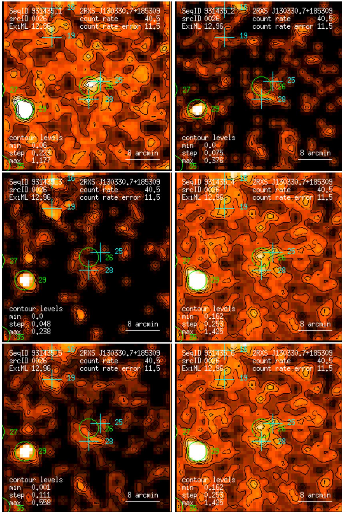
Figure 26: RASS 931435: detection 0026: band rate images, Gaussian filter: (1) PSPC channels 11 – 41, (2) 52 – 90, (3) 91 – 201, (4) 11 – 235, (5) 52 – 201, (6) 11 – 201. Broad band rates in counts/ks. Band rate contour levels in counts/ks/arcmin 2 .
