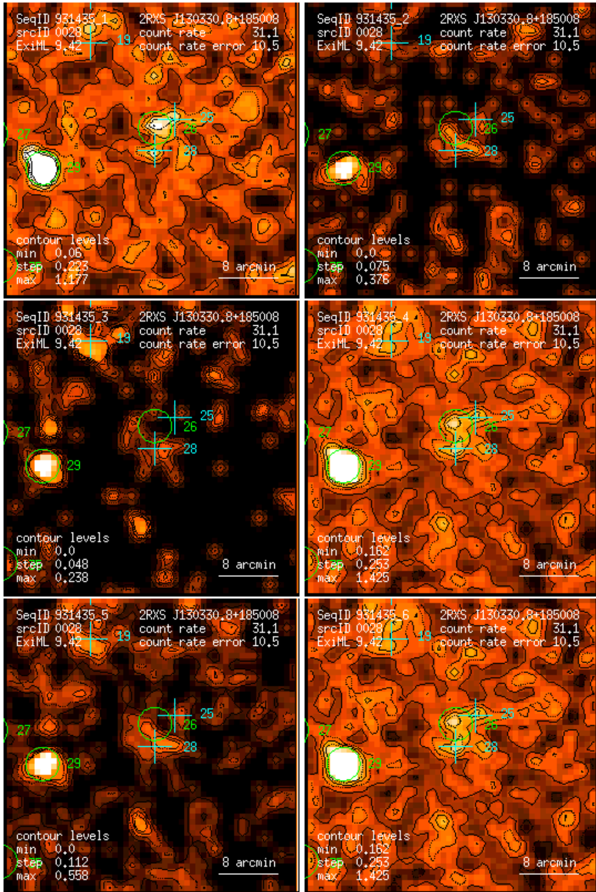
Figure 28: RASS 931435: detection 0028: band rate images, Gaussian filter: (1) PSPC channels 11 – 41, (2) 52 – 90, (3) 91 – 201, (4) 11 – 235, (5) 52 – 201, (6) 11 – 201. Broad band rates in counts/ks. Band rate contour levels in counts/ks/arcmin 2 .
