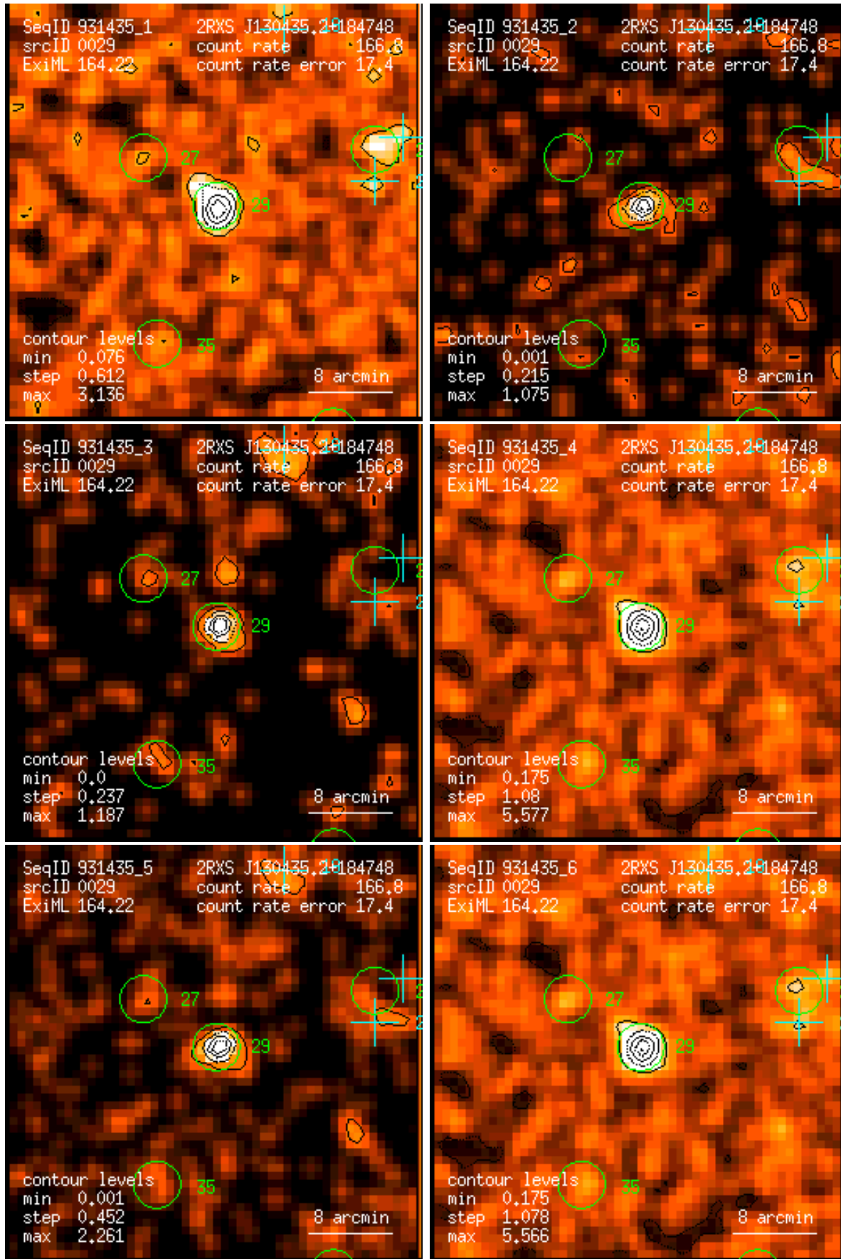
Figure 29: RASS 931435: detection 0029: band rate images, Gaussian filter: (1) PSPC channels 11 – 41, (2) 52 – 90, (3) 91 – 201, (4) 11 – 235, (5) 52 – 201, (6) 11 – 201. Broad band rates in counts/ks. Band rate contour levels in counts/ks/arcmin 2 .
