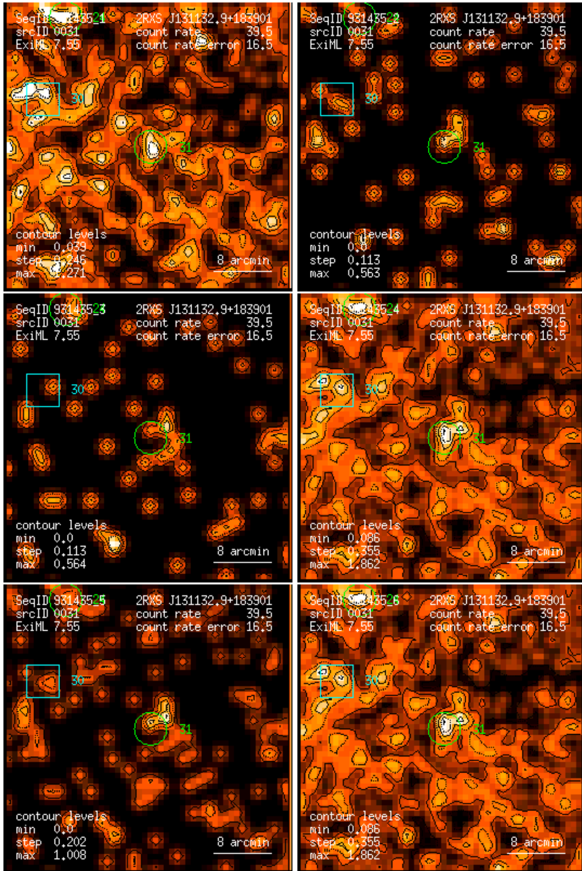
Figure 31: RASS 931435: detection 0031: band rate images, Gaussian filter: (1) PSPC channels 11 – 41, (2) 52 – 90, (3) 91 – 201, (4) 11 – 235, (5) 52 – 201, (6) 11 – 201. Broad band rates in counts/ks. Band rate contour levels in counts/ks/arcmin 2 .
